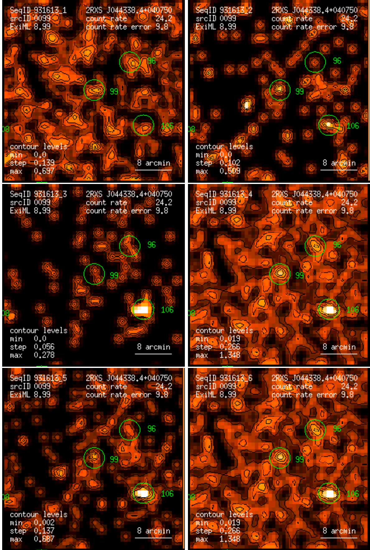
Figure 99: RASS 931613: detection 0099: band rate images, Gaussian filter: (1) PSPC channels 11 – 41, (2) 52 – 90, (3) 91 – 201, (4) 11 – 235, (5) 52 – 201, (6) 11 – 201. Broad band rates in counts/ks. Band rate contour levels in counts/ks/arcmin 2 .
