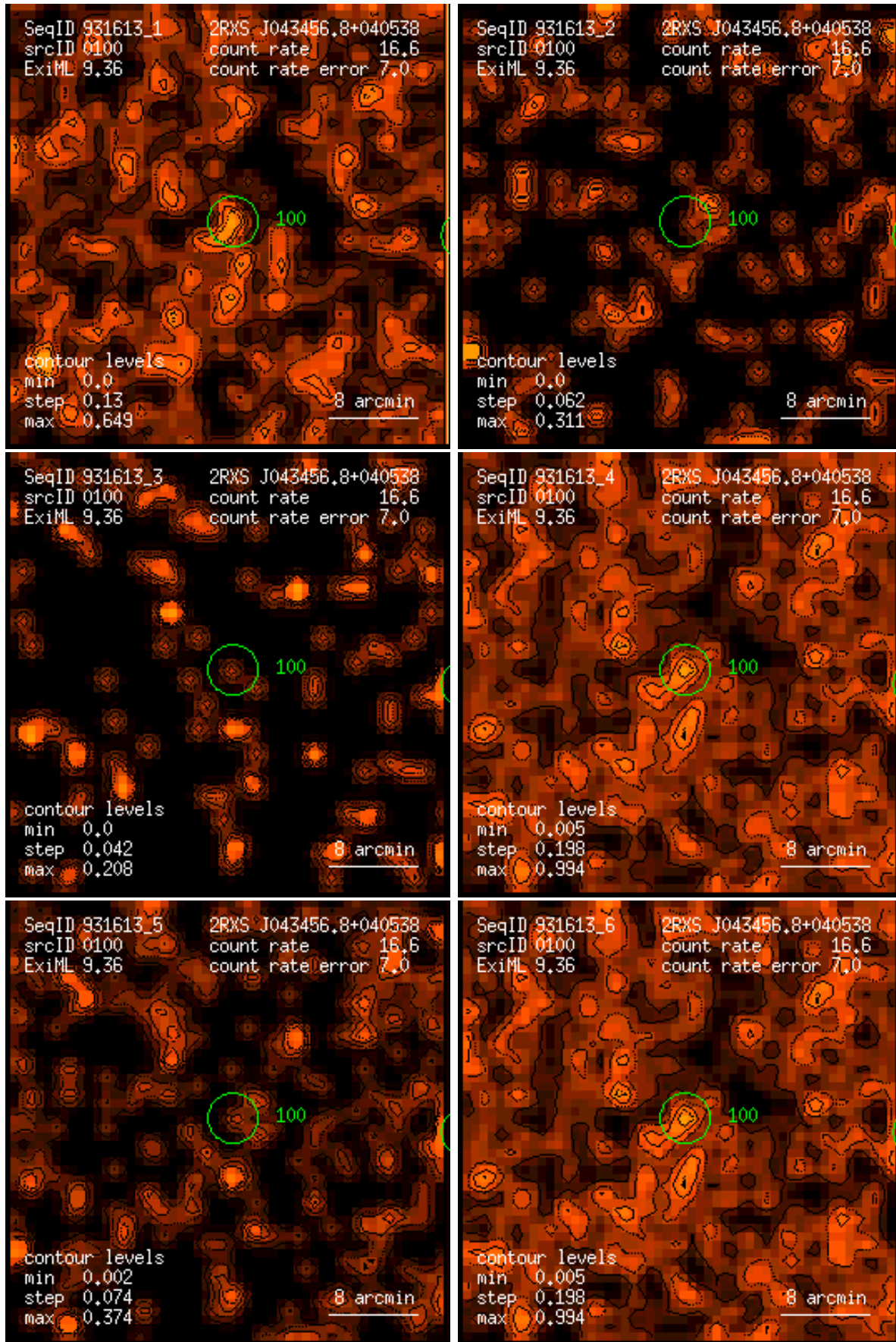
Figure 100: RASS 931613: detection 0100: band rate images, Gaussian filter: (1) PSPC channels 11 – 41, (2) 52 – 90, (3) 91 – 201, (4) 11 – 235, (5) 52 – 201, (6) 11 – 201. Broad band rates in counts/ks. Band rate contour levels in counts/ks/arcmin 2 .
