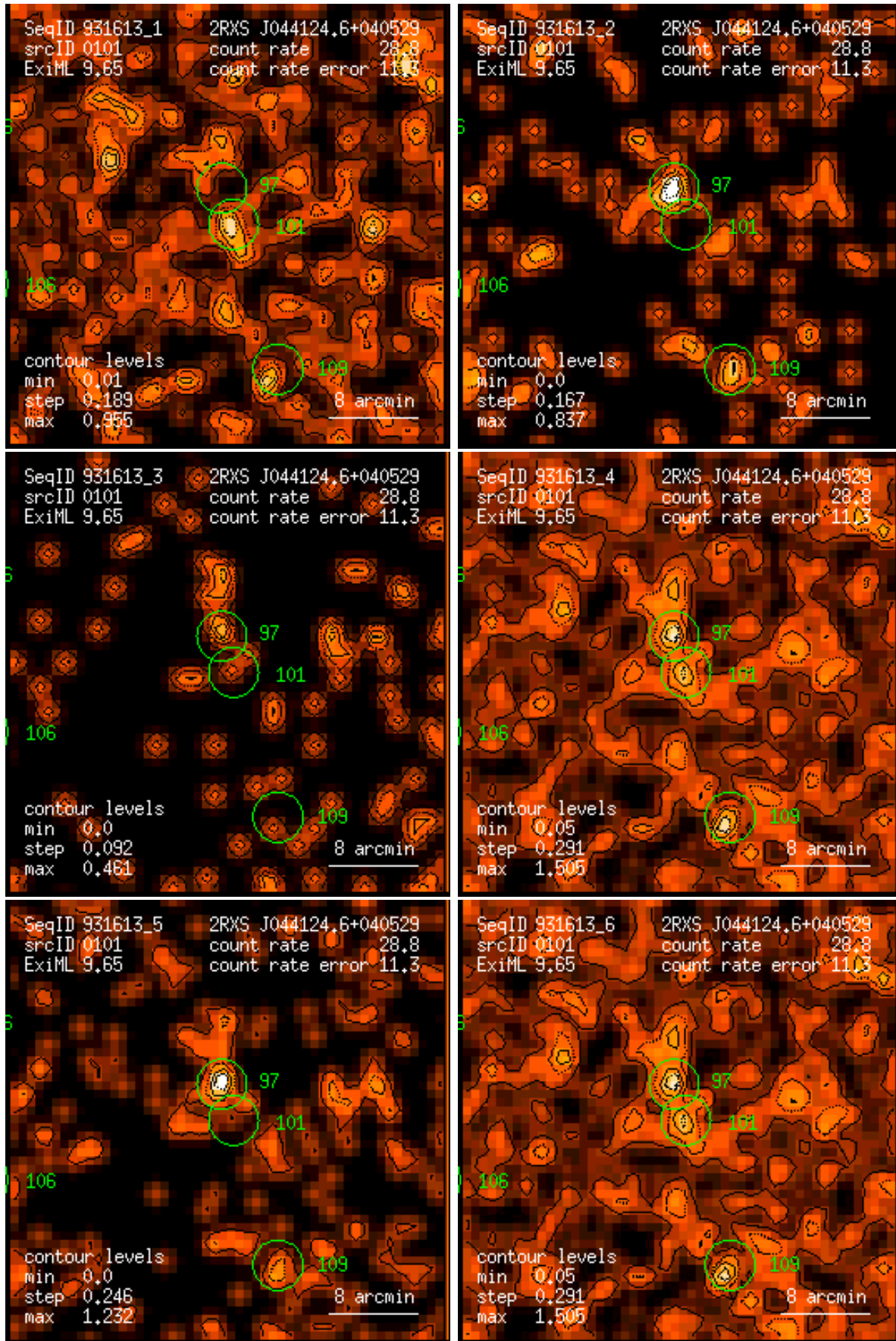
Figure 101: RASS 931613: detection 0101: band rate images, Gaussian filter: (1) PSPC channels 11 – 41, (2) 52 – 90, (3) 91 – 201, (4) 11 – 235, (5) 52 – 201, (6) 11 – 201. Broad band rates in counts/ks. Band rate contour levels in counts/ks/arcmin 2 .
