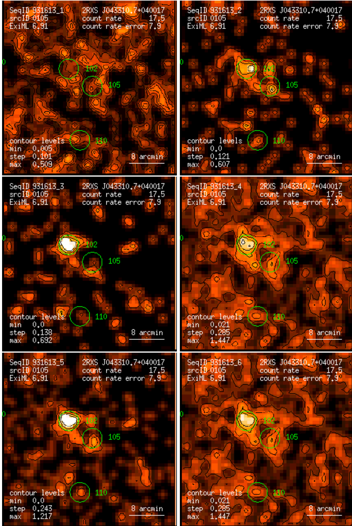
Figure 105: RASS 931613: detection 0105: band rate images, Gaussian filter: (1) PSPC channels 11 – 41, (2) 52 – 90, (3) 91 – 201, (4) 11 – 235, (5) 52 – 201, (6) 11 – 201. Broad band rates in counts/ks. Band rate contour levels in counts/ks/arcmin 2 .
