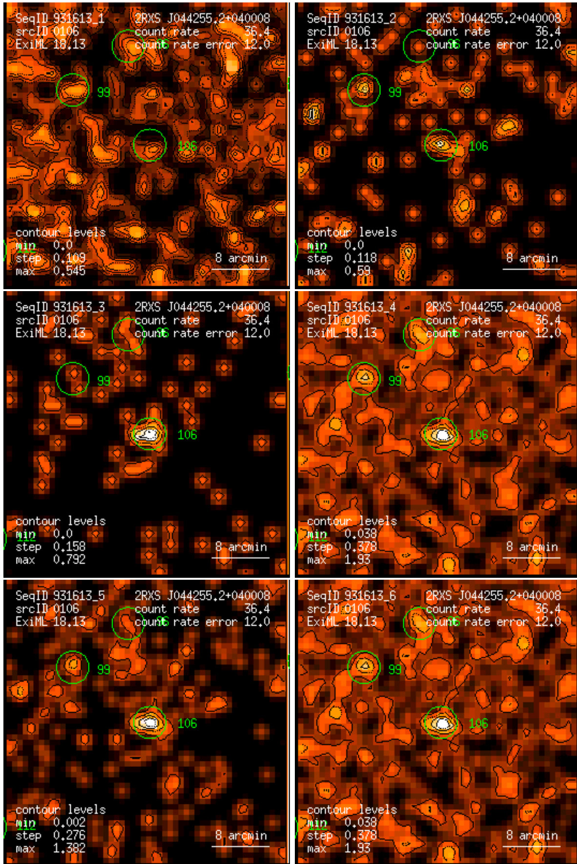
Figure 106: RASS 931613: detection 0106: band rate images, Gaussian filter: (1) PSPC channels 11 – 41, (2) 52 – 90, (3) 91 – 201, (4) 11 – 235, (5) 52 – 201, (6) 11 – 201. Broad band rates in counts/ks. Band rate contour levels in counts/ks/arcmin 2 .
