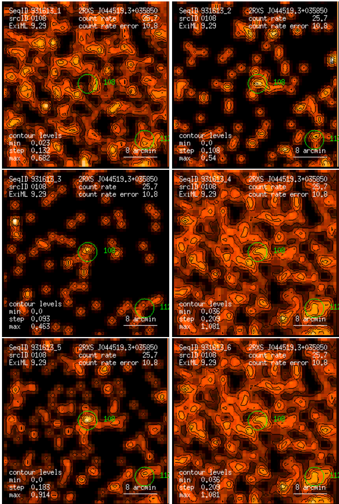
Figure 108: RASS 931613: detection 0108: band rate images, Gaussian filter: (1) PSPC channels 11 – 41, (2) 52 – 90, (3) 91 – 201, (4) 11 – 235, (5) 52 – 201, (6) 11 – 201. Broad band rates in counts/ks. Band rate contour levels in counts/ks/arcmin 2 .
