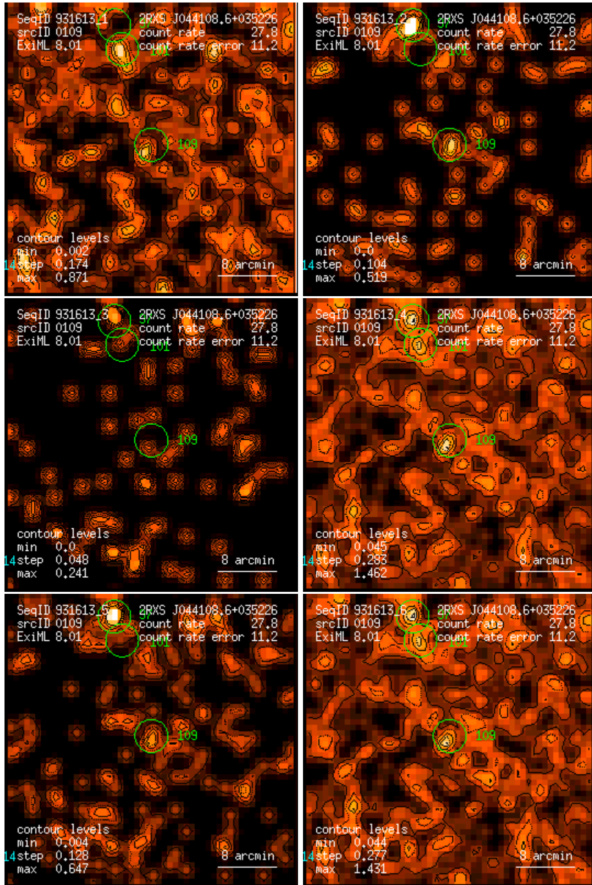
Figure 109: RASS 931613: detection 0109: band rate images, Gaussian filter: (1) PSPC channels 11 – 41, (2) 52 – 90, (3) 91 – 201, (4) 11 – 235, (5) 52 – 201, (6) 11 – 201. Broad band rates in counts/ks. Band rate contour levels in counts/ks/arcmin 2 .
