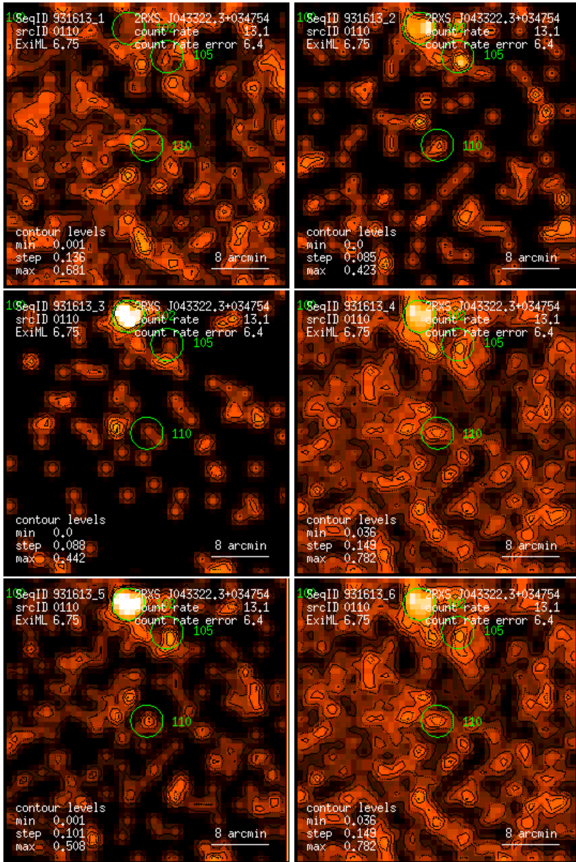
Figure 110: RASS 931613: detection 0110: band rate images, Gaussian filter: (1) PSPC channels 11 – 41, (2) 52 – 90, (3) 91 – 201, (4) 11 – 235, (5) 52 – 201, (6) 11 – 201. Broad band rates in counts/ks. Band rate contour levels in counts/ks/arcmin 2 .
