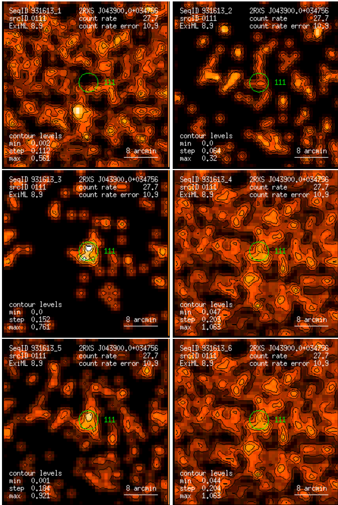
Figure 111: RASS 931613: detection 0111: band rate images, Gaussian filter: (1) PSPC channels 11 – 41, (2) 52 – 90, (3) 91 – 201, (4) 11 – 235, (5) 52 – 201, (6) 11 – 201. Broad band rates in counts/ks. Band rate contour levels in counts/ks/arcmin 2 .
