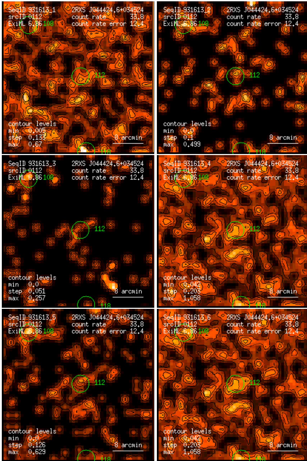
Figure 112: RASS 931613: detection 0112: band rate images, Gaussian filter: (1) PSPC channels 11 – 41, (2) 52 – 90, (3) 91 – 201, (4) 11 – 235, (5) 52 – 201, (6) 11 – 201. Broad band rates in counts/ks. Band rate contour levels in counts/ks/arcmin 2 .
