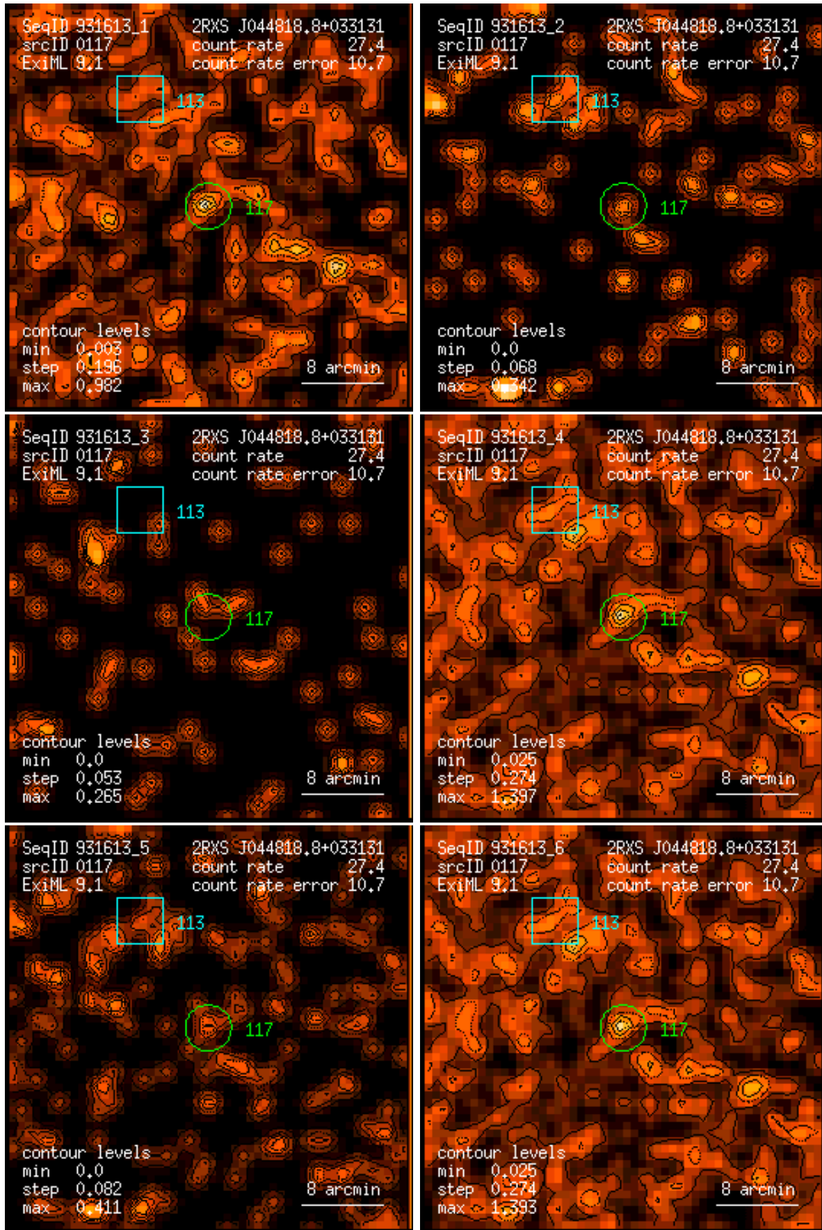
Figure 117: RASS 931613: detection 0117: band rate images, Gaussian filter: (1) PSPC channels 11 – 41, (2) 52 – 90, (3) 91 – 201, (4) 11 – 235, (5) 52 – 201, (6) 11 – 201. Broad band rates in counts/ks. Band rate contour levels in counts/ks/arcmin 2 .
