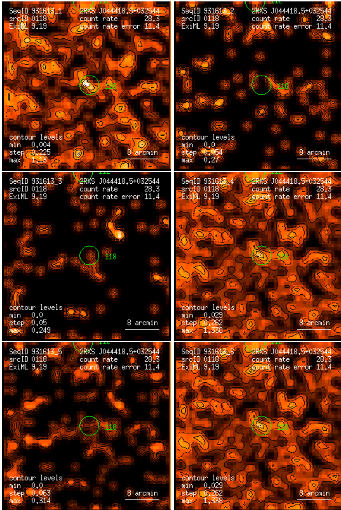
Figure 118: RASS 931613: detection 0118: band rate images, Gaussian filter: (1) PSPC channels 11 – 41, (2) 52 – 90, (3) 91 – 201, (4) 11 – 235, (5) 52 – 201, (6) 11 – 201. Broad band rates in counts/ks. Band rate contour levels in counts/ks/arcmin 2 .
