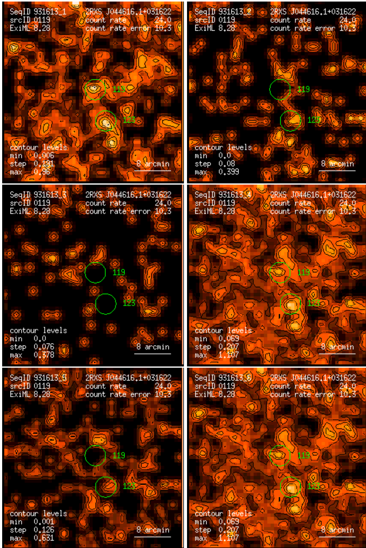
Figure 119: RASS 931613: detection 0119: band rate images, Gaussian filter: (1) PSPC channels 11 – 41, (2) 52 – 90, (3) 91 – 201, (4) 11 – 235, (5) 52 – 201, (6) 11 – 201. Broad band rates in counts/ks. Band rate contour levels in counts/ks/arcmin 2 .
