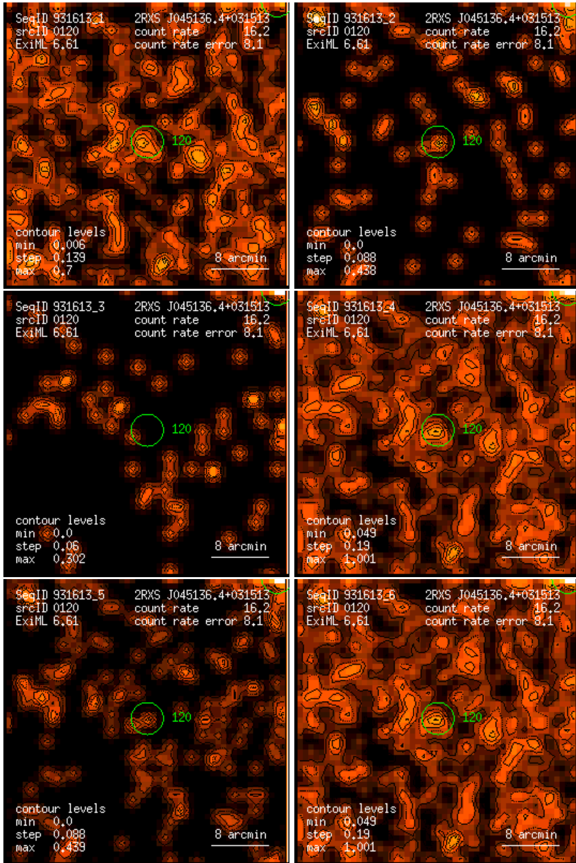
Figure 120: RASS 931613: detection 0120: band rate images, Gaussian filter: (1) PSPC channels 11 – 41, (2) 52 – 90, (3) 91 – 201, (4) 11 – 235, (5) 52 – 201, (6) 11 – 201. Broad band rates in counts/ks. Band rate contour levels in counts/ks/arcmin 2 .
