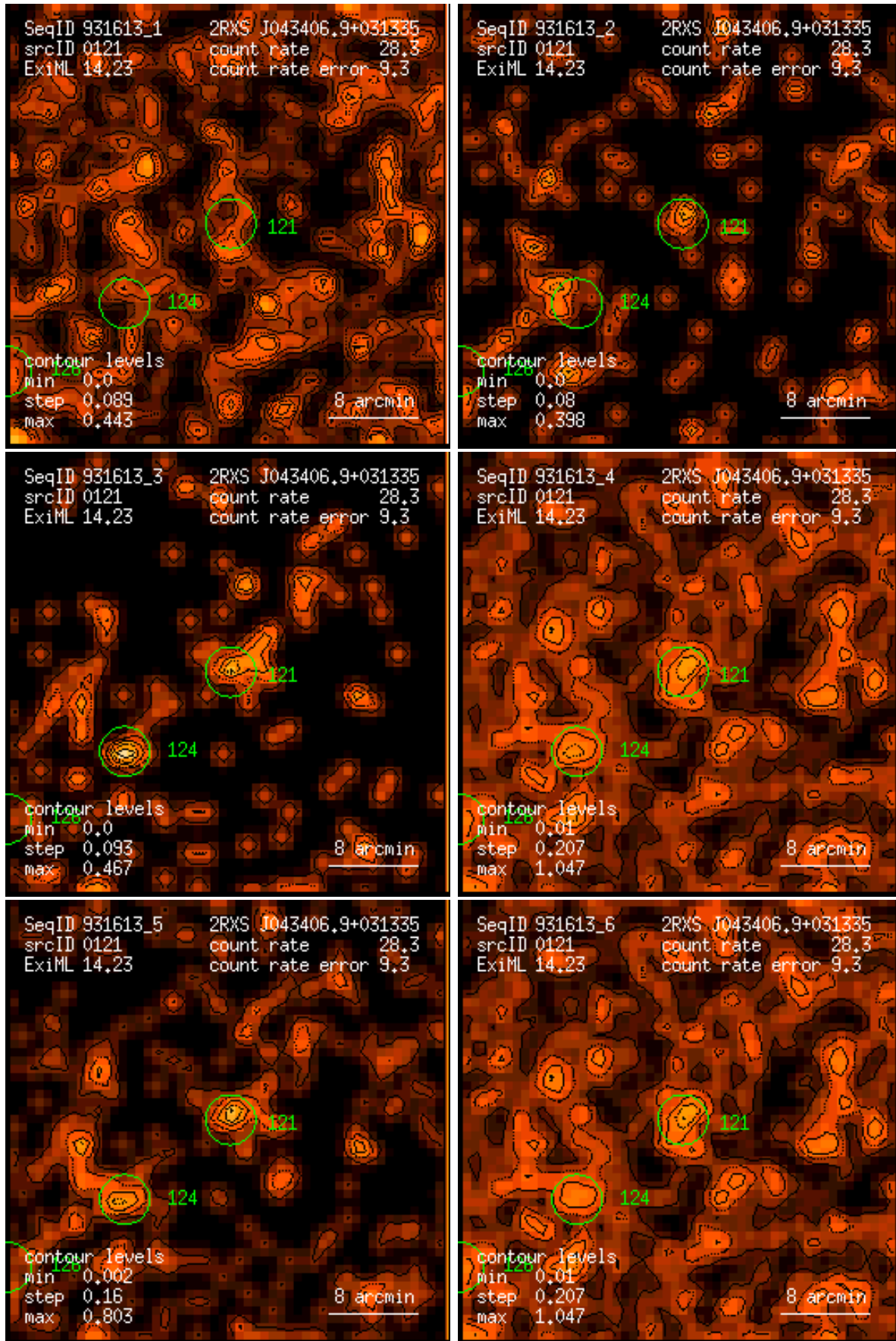
Figure 121: RASS 931613: detection 0121: band rate images, Gaussian filter: (1) PSPC channels 11 – 41, (2) 52 – 90, (3) 91 – 201, (4) 11 – 235, (5) 52 – 201, (6) 11 – 201. Broad band rates in counts/ks. Band rate contour levels in counts/ks/arcmin 2 .
