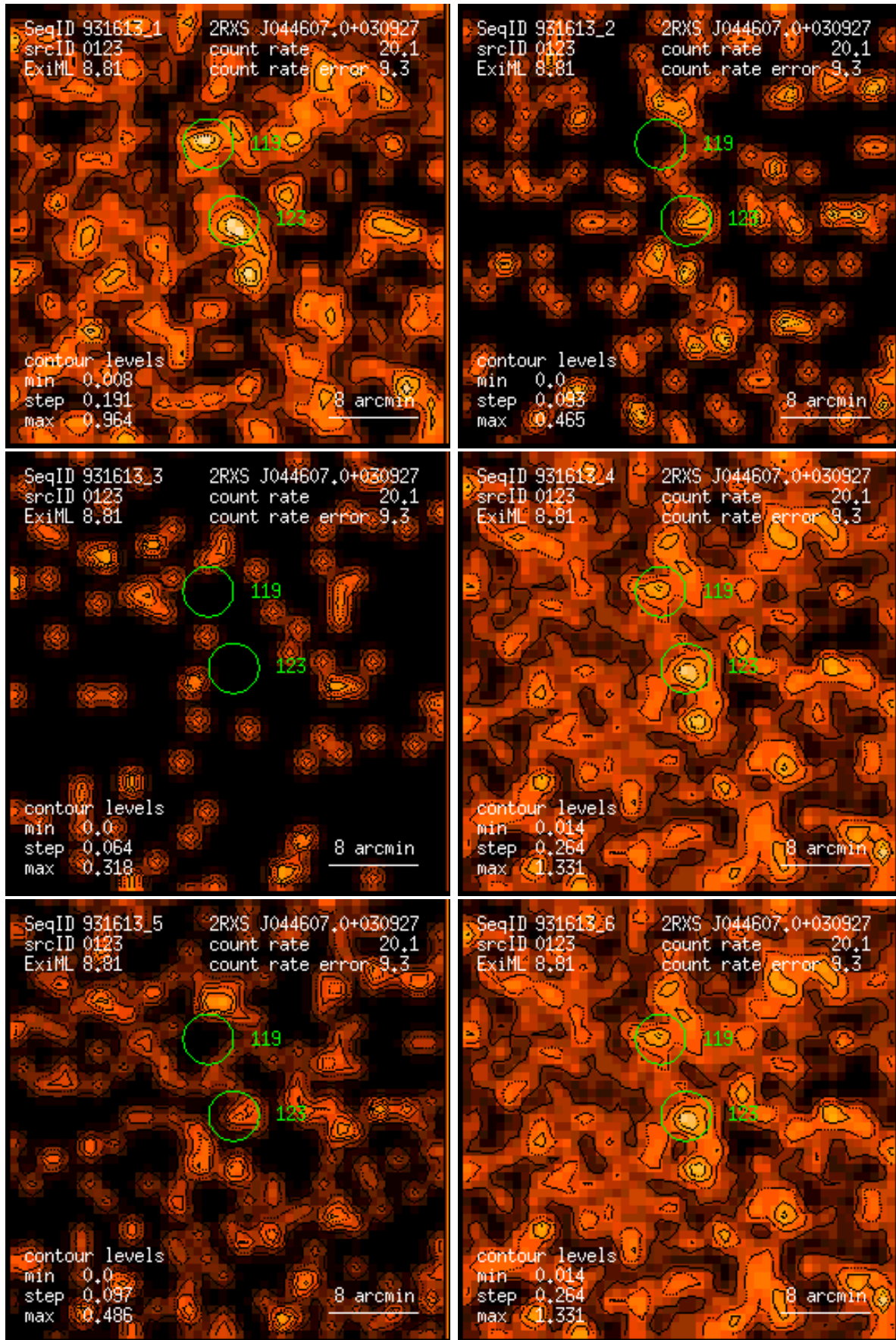
Figure 123: RASS 931613: detection 0123: band rate images, Gaussian filter: (1) PSPC channels 11 – 41, (2) 52 – 90, (3) 91 – 201, (4) 11 – 235, (5) 52 – 201, (6) 11 – 201. Broad band rates in counts/ks. Band rate contour levels in counts/ks/arcmin 2 .
