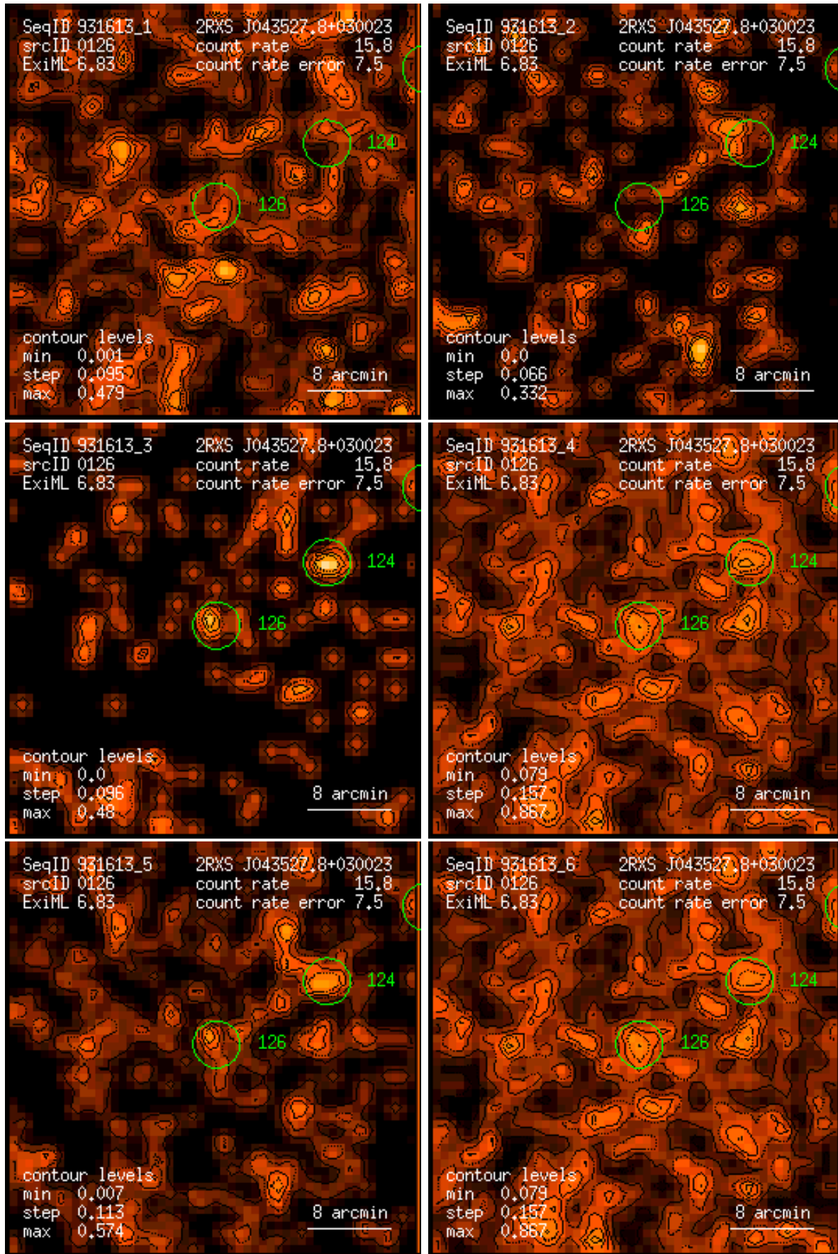
Figure 126: RASS 931613: detection 0126: band rate images, Gaussian filter: (1) PSPC channels 11 – 41, (2) 52 – 90, (3) 91 – 201, (4) 11 – 235, (5) 52 – 201, (6) 11 – 201. Broad band rates in counts/ks. Band rate contour levels in counts/ks/arcmin 2 .
