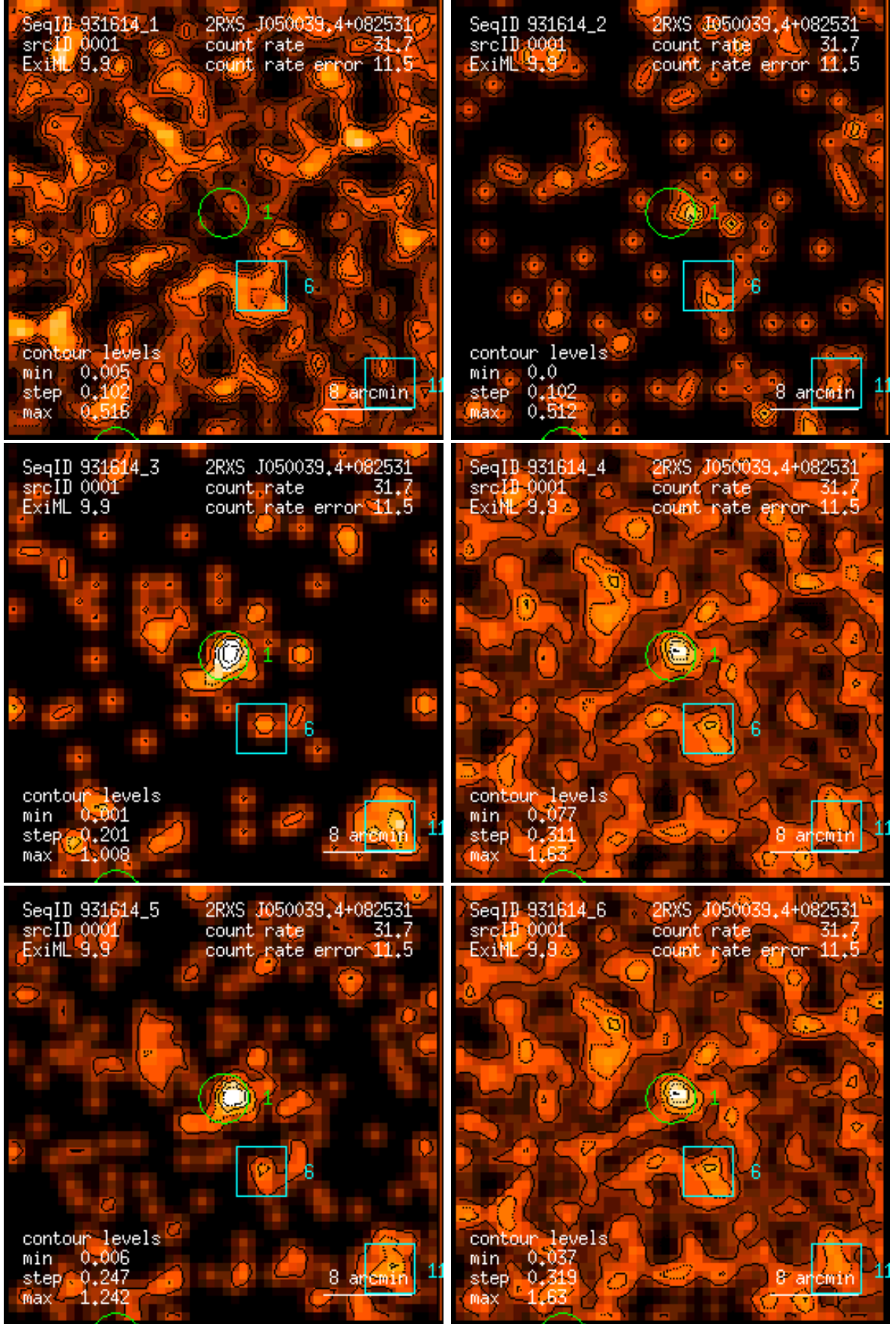
Figure 1: RASS 931614: detection 0001: band rate images, Gaussian filter: (1) PSPC channels 11 – 41, (2) 52 – 90, (3) 91 – 201, (4) 11 – 235, (5) 52 – 201, (6) 11 – 201. Broad band rates in counts/ks. Band rate contour levels in counts/ks/arcmin 2 .
