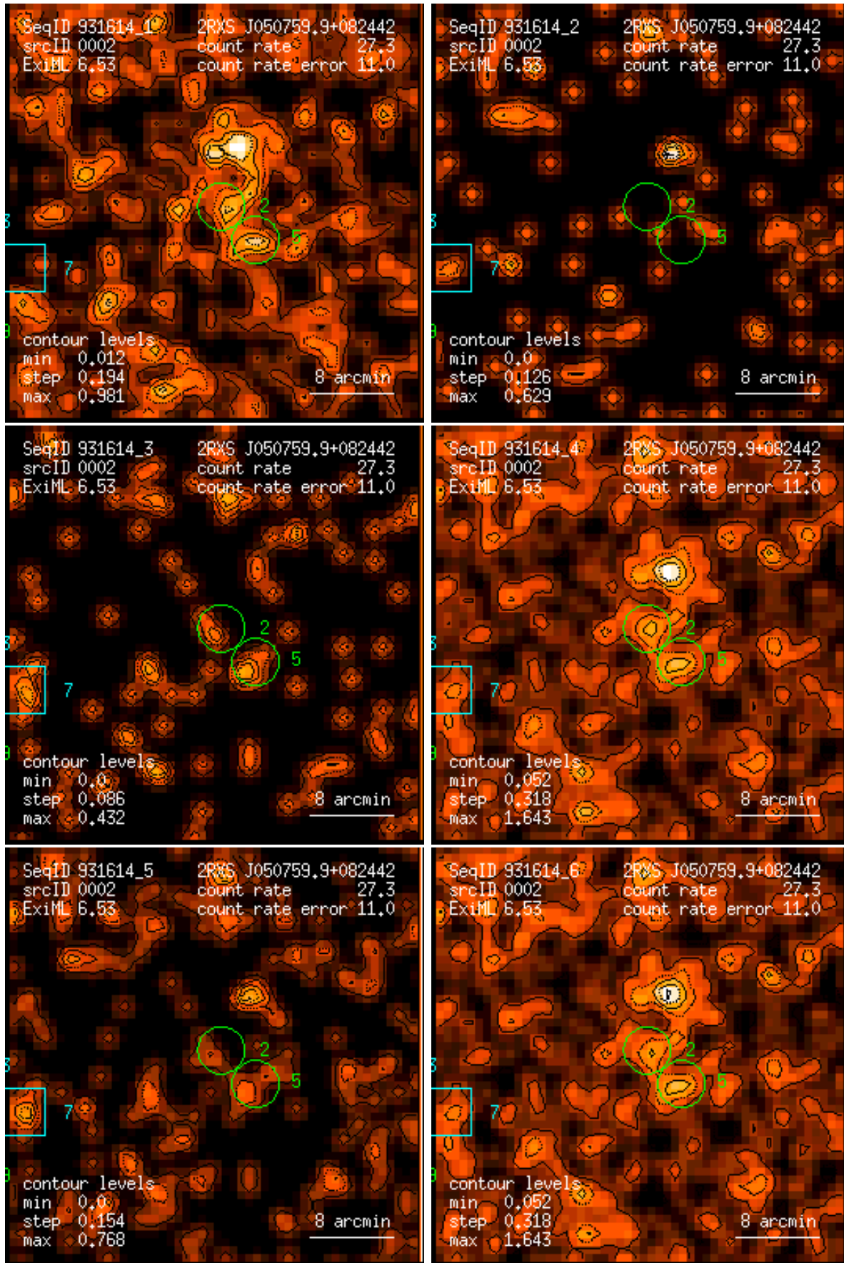
Figure 2: RASS 931614: detection 0002: band rate images, Gaussian filter: (1) PSPC channels 11 – 41, (2) 52 – 90, (3) 91 – 201, (4) 11 – 235, (5) 52 – 201, (6) 11 – 201. Broad band rates in counts/ks. Band rate contour levels in counts/ks/arcmin 2 .
