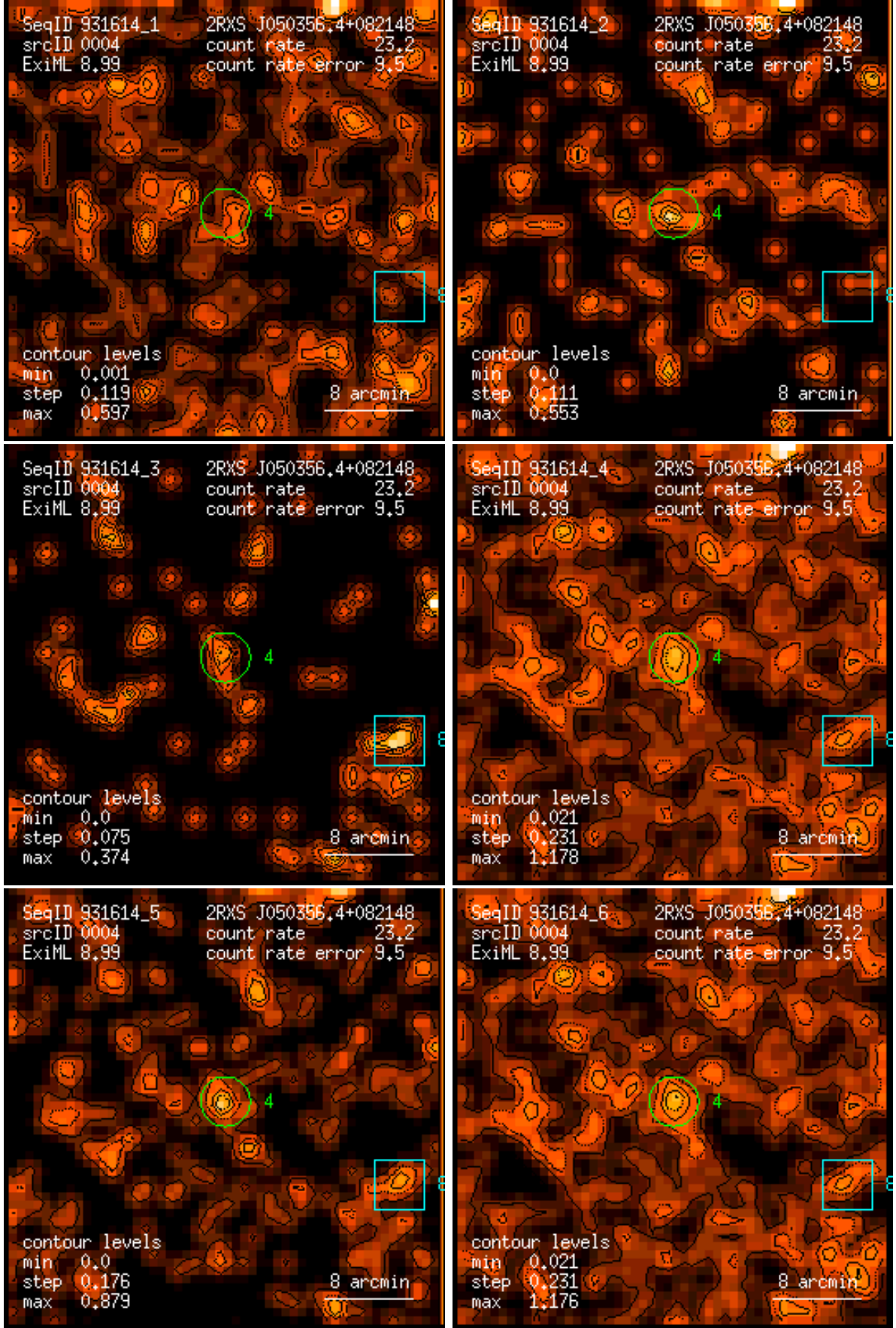
Figure 4: RASS 931614: detection 0004: band rate images, Gaussian filter: (1) PSPC channels 11 – 41, (2) 52 – 90, (3) 91 – 201, (4) 11 – 235, (5) 52 – 201, (6) 11 – 201. Broad band rates in counts/ks. Band rate contour levels in counts/ks/arcmin 2 .
