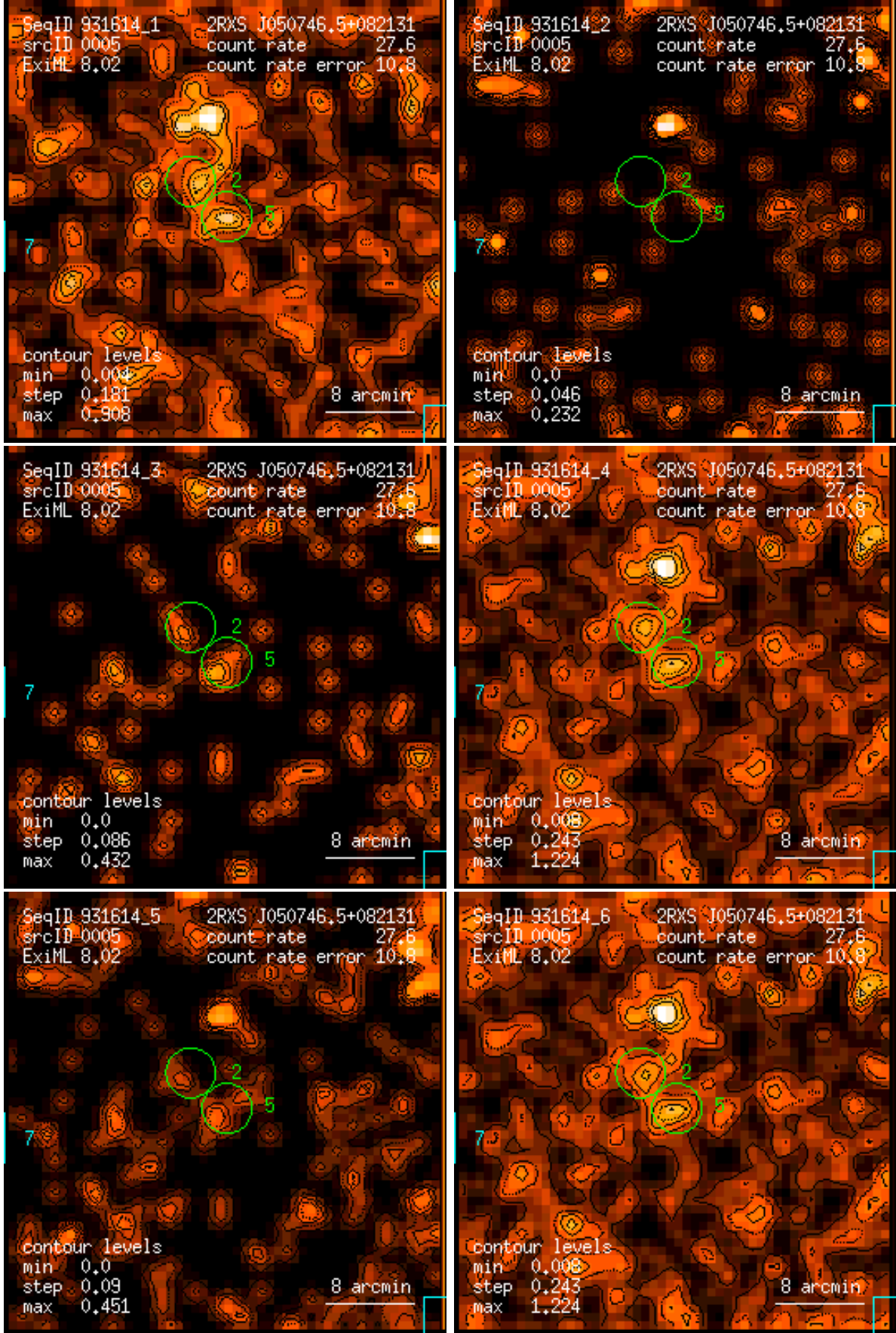
Figure 5: RASS 931614: detection 0005: band rate images, Gaussian filter: (1) PSPC channels 11 – 41, (2) 52 – 90, (3) 91 – 201, (4) 11 – 235, (5) 52 – 201, (6) 11 – 201. Broad band rates in counts/ks. Band rate contour levels in counts/ks/arcmin 2 .
