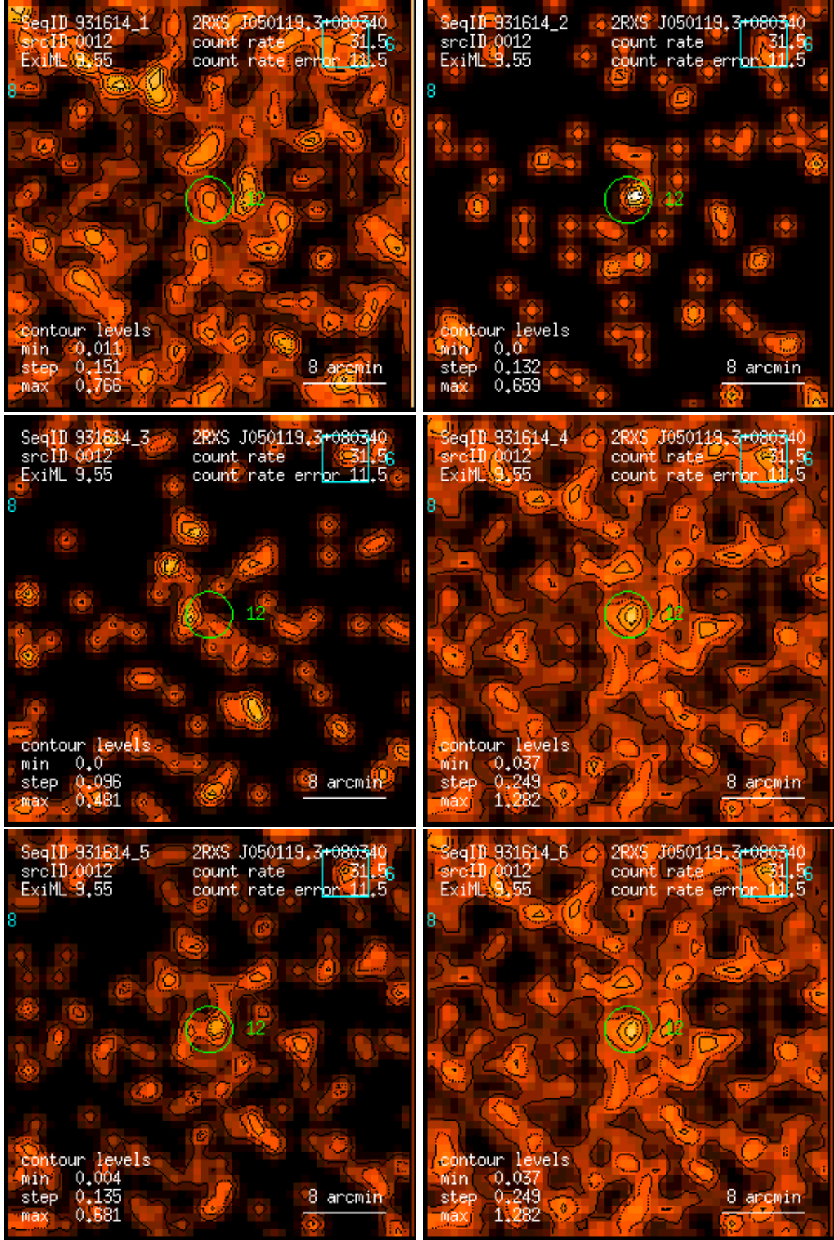
Figure 12: RASS 931614: detection 0012: band rate images, Gaussian filter: (1) PSPC channels 11 – 41, (2) 52 – 90, (3) 91 – 201, (4) 11 – 235, (5) 52 – 201, (6) 11 – 201. Broad band rates in counts/ks. Band rate contour levels in counts/ks/arcmin 2 .
