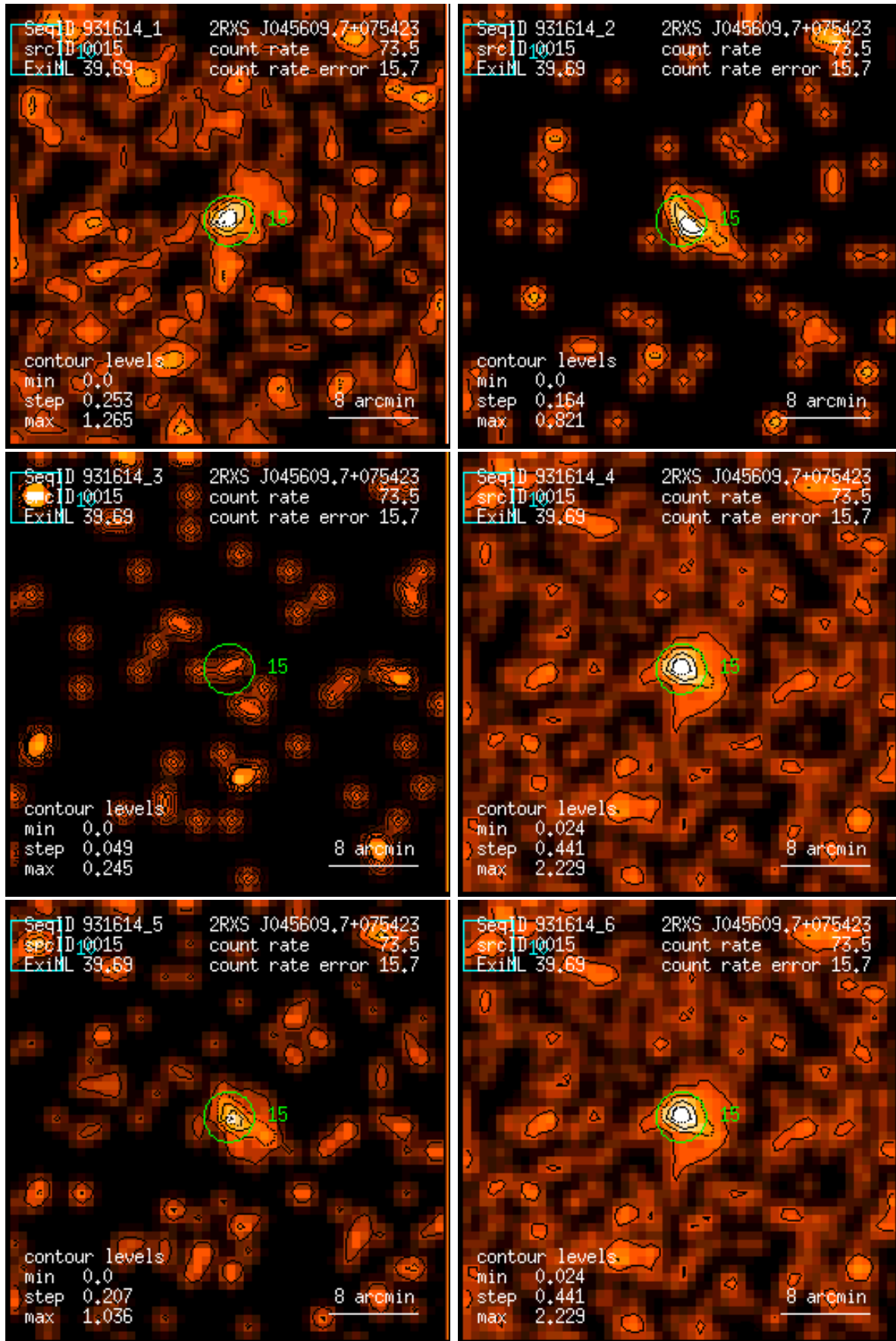
Figure 15: RASS 931614: detection 0015: band rate images, Gaussian filter: (1) PSPC channels 11 – 41, (2) 52 – 90, (3) 91 – 201, (4) 11 – 235, (5) 52 – 201, (6) 11 – 201. Broad band rates in counts/ks. Band rate contour levels in counts/ks/arcmin 2 .
