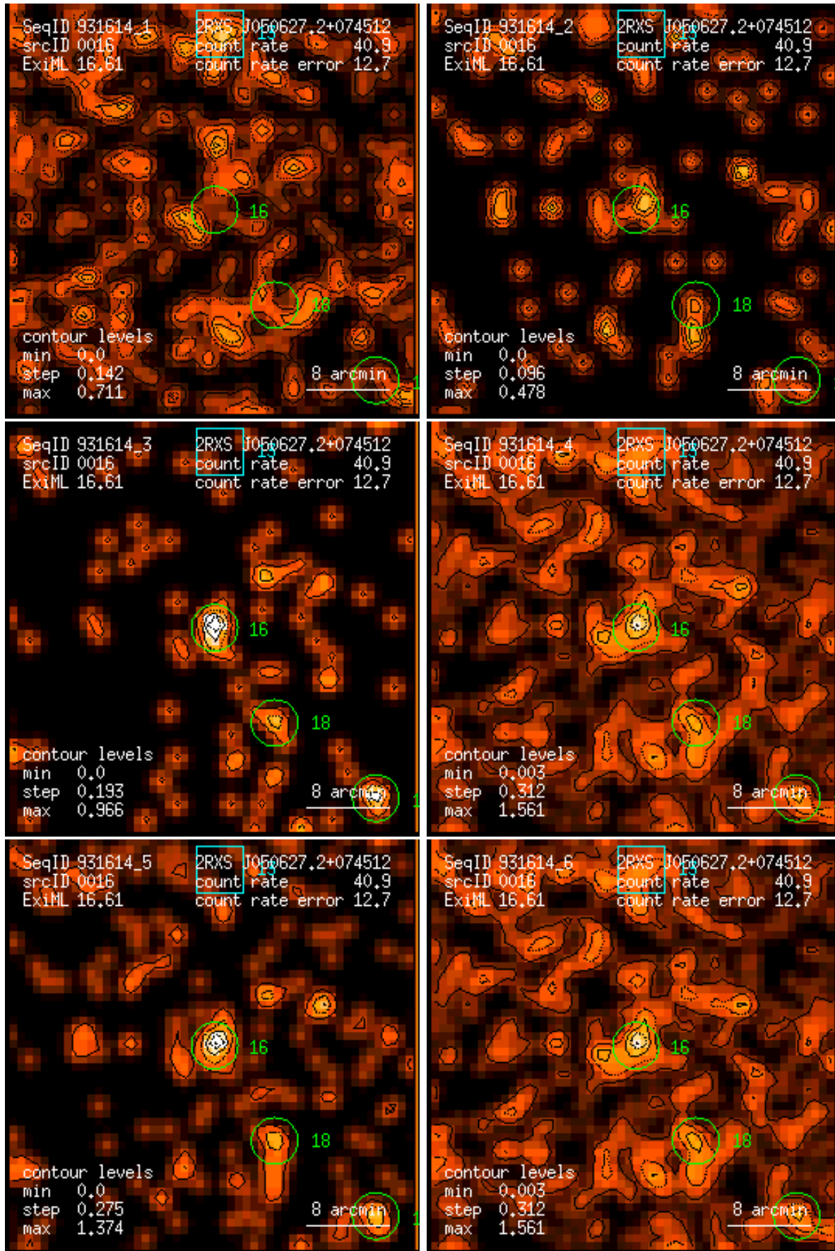
Figure 16: RASS 931614: detection 0016: band rate images, Gaussian filter: (1) PSPC channels 11 – 41, (2) 52 – 90, (3) 91 – 201, (4) 11 – 235, (5) 52 – 201, (6) 11 – 201. Broad band rates in counts/ks. Band rate contour levels in counts/ks/arcmin 2 .
