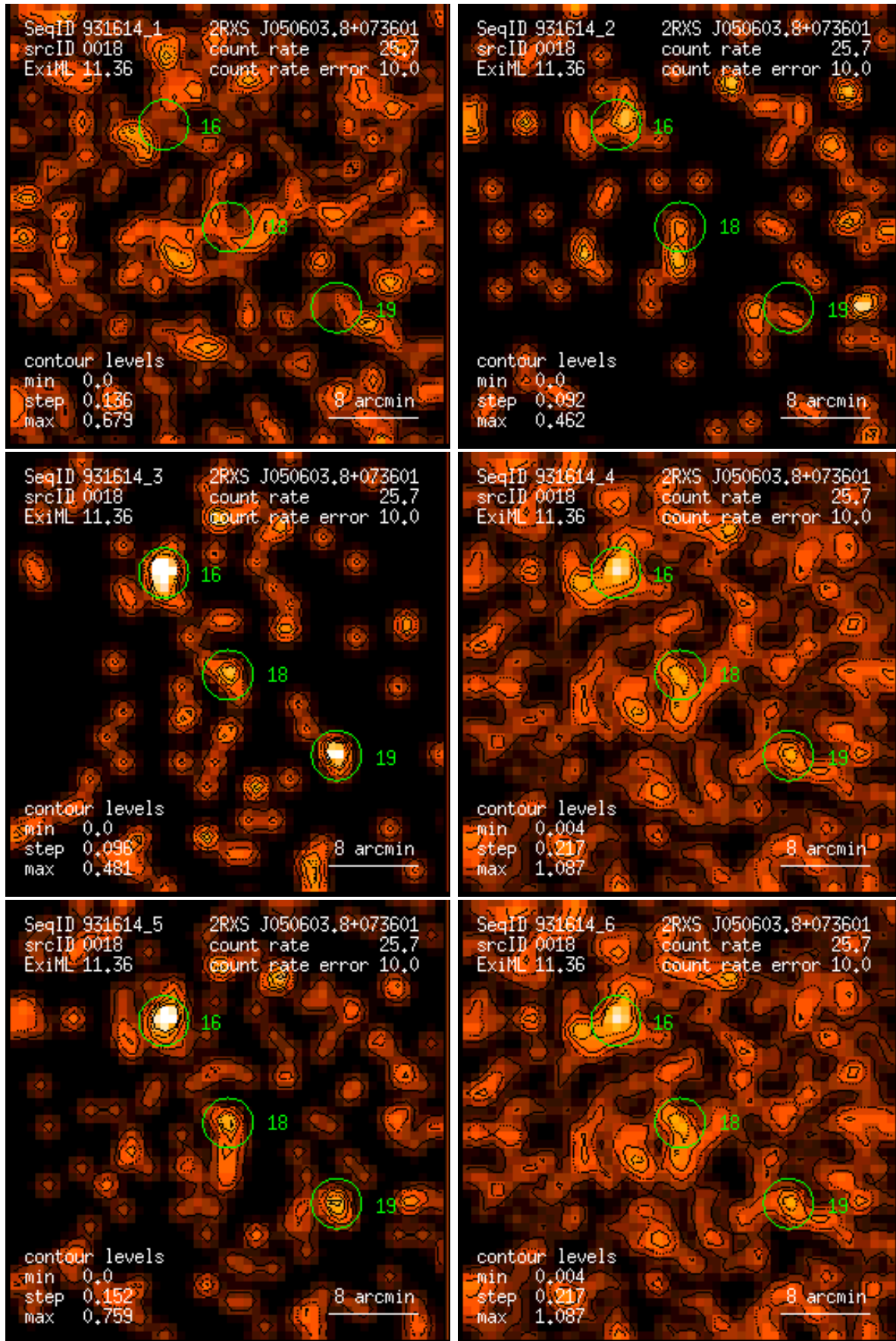
Figure 18: RASS 931614: detection 0018: band rate images, Gaussian filter: (1) PSPC channels 11 – 41, (2) 52 – 90, (3) 91 – 201, (4) 11 – 235, (5) 52 – 201, (6) 11 – 201. Broad band rates in counts/ks. Band rate contour levels in counts/ks/arcmin 2 .
