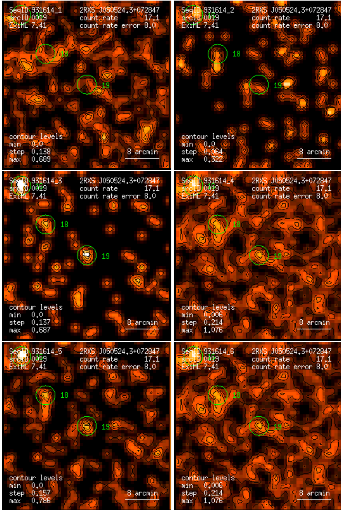
Figure 19: RASS 931614: detection 0019: band rate images, Gaussian filter: (1) PSPC channels 11 – 41, (2) 52 – 90, (3) 91 – 201, (4) 11 – 235, (5) 52 – 201, (6) 11 – 201. Broad band rates in counts/ks. Band rate contour levels in counts/ks/arcmin 2 .
