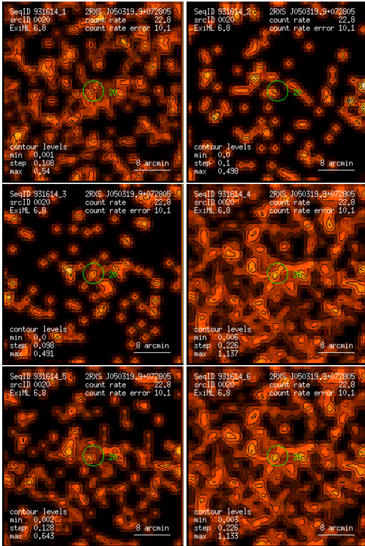
Figure 20: RASS 931614: detection 0020: band rate images, Gaussian filter: (1) PSPC channels 11 – 41, (2) 52 – 90, (3) 91 – 201, (4) 11 – 235, (5) 52 – 201, (6) 11 – 201. Broad band rates in counts/ks. Band rate contour levels in counts/ks/arcmin 2 .
