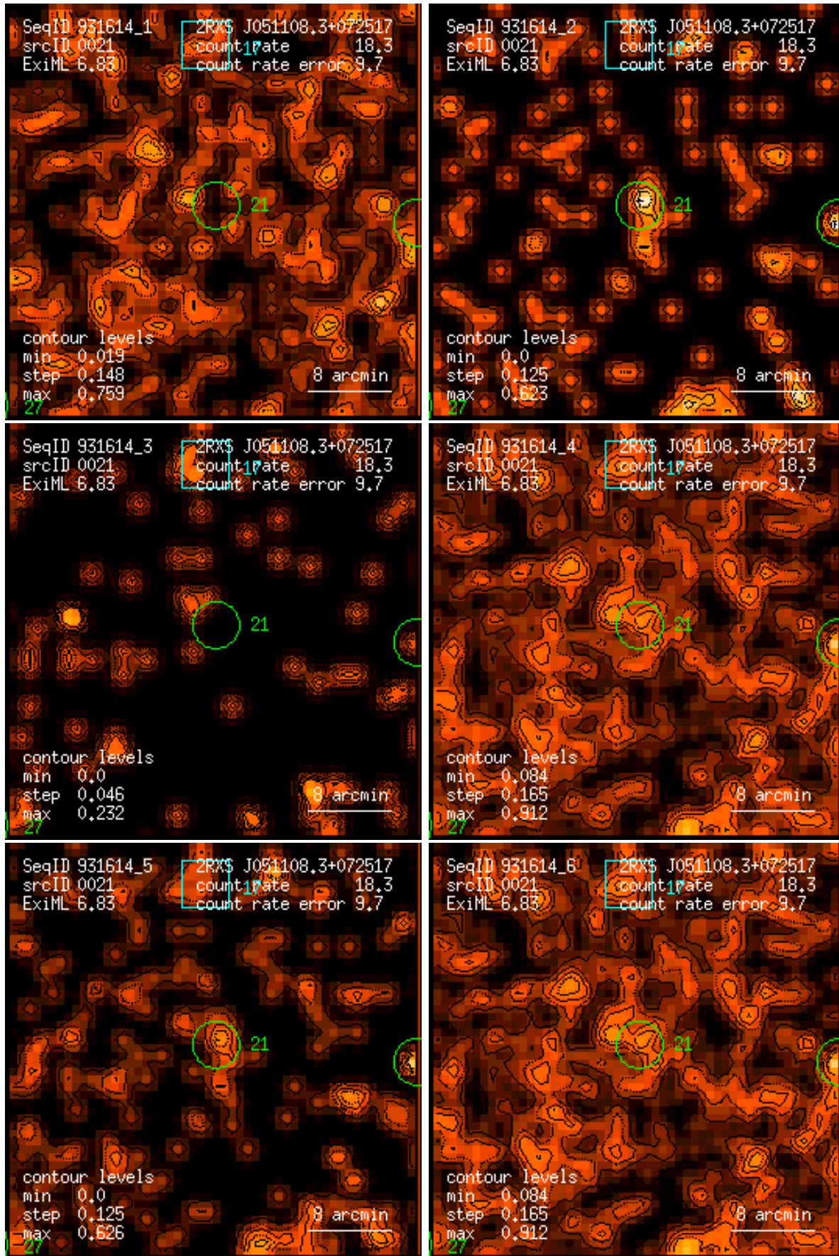
Figure 21: RASS 931614: detection 0021: band rate images, Gaussian filter: (1) PSPC channels 11 – 41, (2) 52 – 90, (3) 91 – 201, (4) 11 – 235, (5) 52 – 201, (6) 11 – 201. Broad band rates in counts/ks. Band rate contour levels in counts/ks/arcmin 2 .
