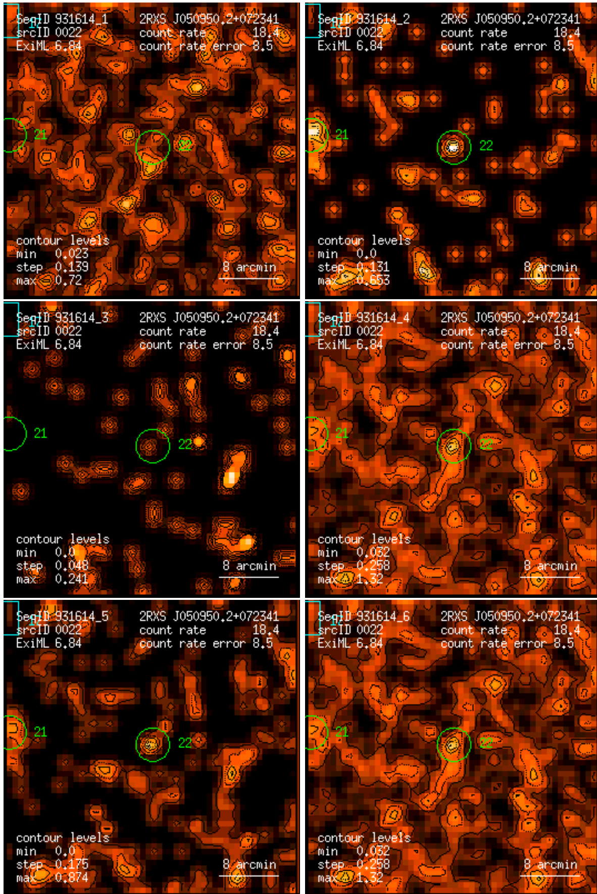
Figure 22: RASS 931614: detection 0022: band rate images, Gaussian filter: (1) PSPC channels 11 – 41, (2) 52 – 90, (3) 91 – 201, (4) 11 – 235, (5) 52 – 201, (6) 11 – 201. Broad band rates in counts/ks. Band rate contour levels in counts/ks/arcmin 2 .
