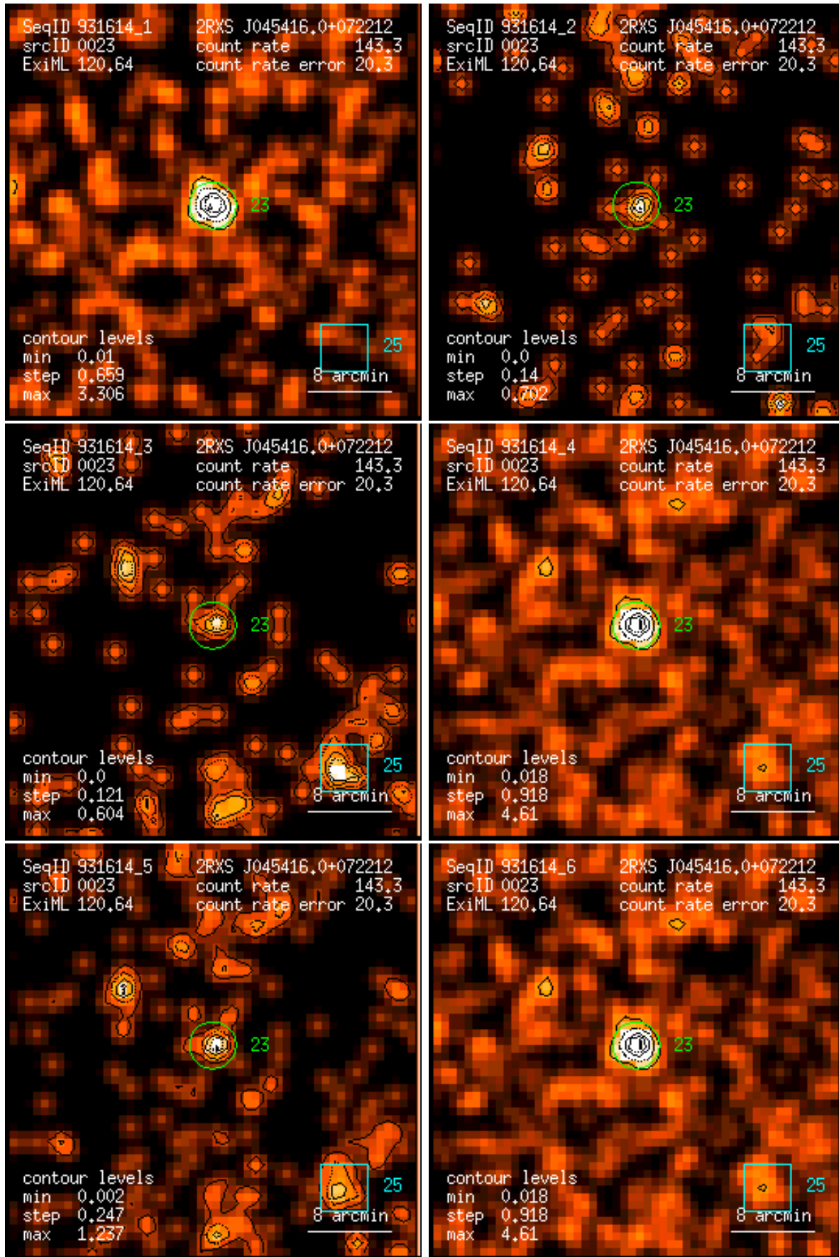
Figure 23: RASS 931614: detection 0023: band rate images, Gaussian filter: (1) PSPC channels 11 – 41, (2) 52 – 90, (3) 91 – 201, (4) 11 – 235, (5) 52 – 201, (6) 11 – 201. Broad band rates in counts/ks. Band rate contour levels in counts/ks/arcmin 2 .
