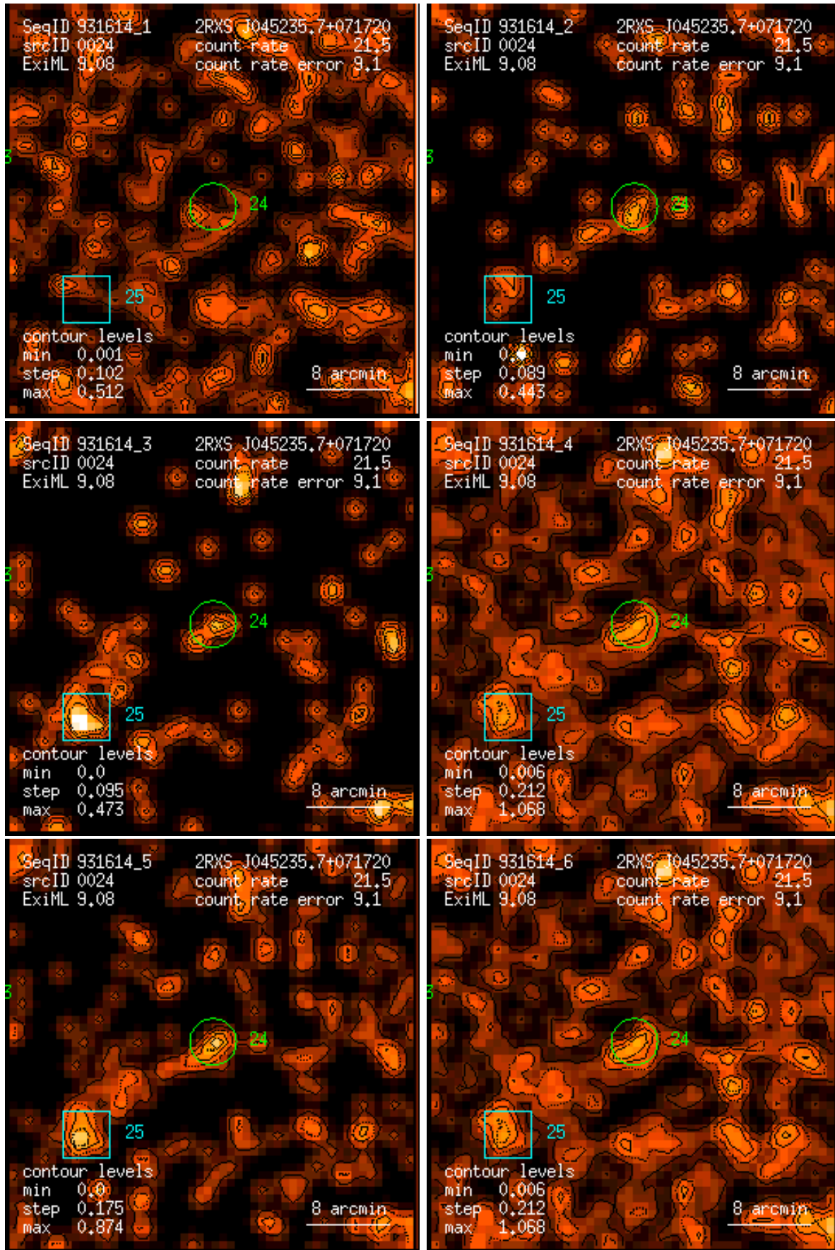
Figure 24: RASS 931614: detection 0024: band rate images, Gaussian filter: (1) PSPC channels 11 – 41, (2) 52 – 90, (3) 91 – 201, (4) 11 – 235, (5) 52 – 201, (6) 11 – 201. Broad band rates in counts/ks. Band rate contour levels in counts/ks/arcmin 2 .
