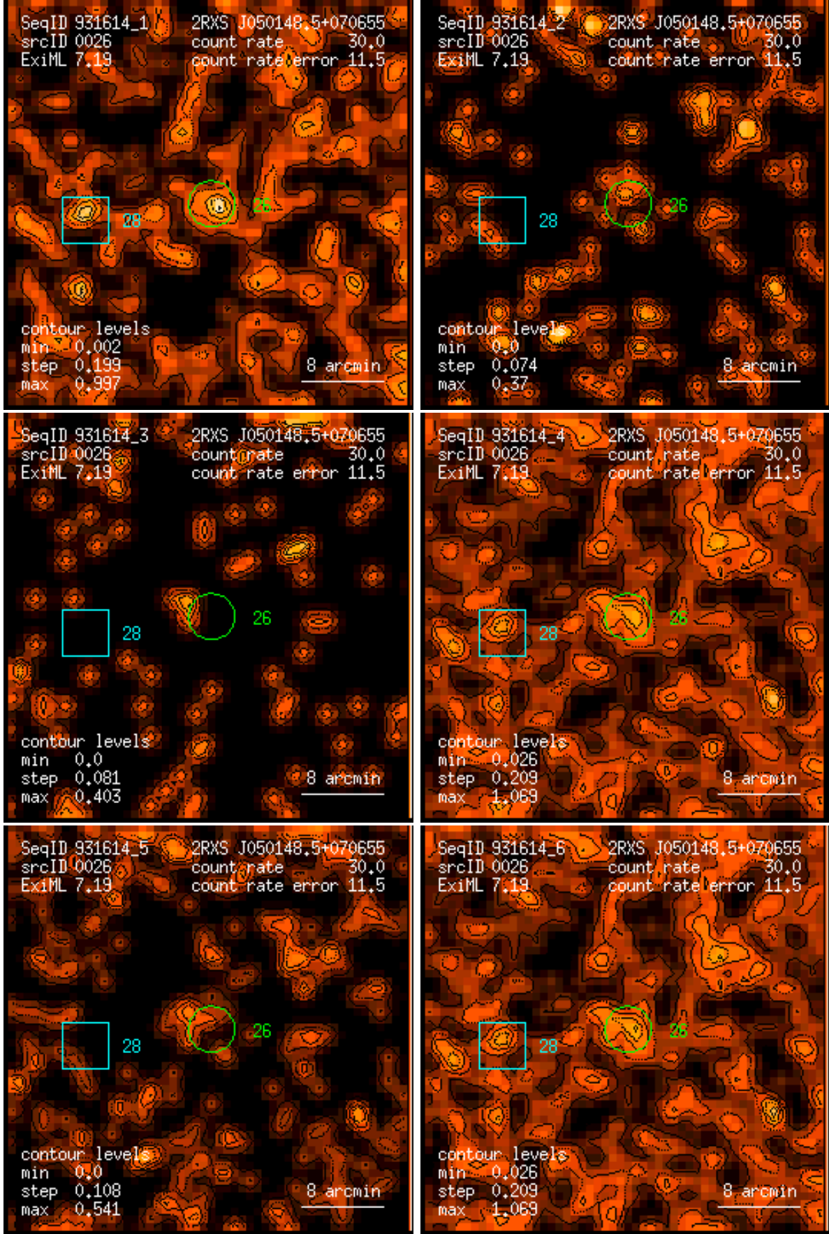
Figure 26: RASS 931614: detection 0026: band rate images, Gaussian filter: (1) PSPC channels 11 – 41, (2) 52 – 90, (3) 91 – 201, (4) 11 – 235, (5) 52 – 201, (6) 11 – 201. Broad band rates in counts/ks. Band rate contour levels in counts/ks/arcmin 2 .
