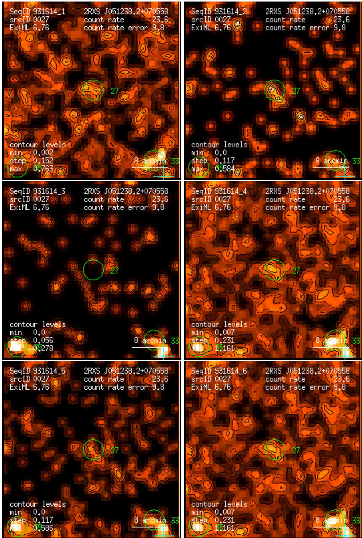
Figure 27: RASS 931614: detection 0027: band rate images, Gaussian filter: (1) PSPC channels 11 – 41, (2) 52 – 90, (3) 91 – 201, (4) 11 – 235, (5) 52 – 201, (6) 11 – 201. Broad band rates in counts/ks. Band rate contour levels in counts/ks/arcmin 2 .
