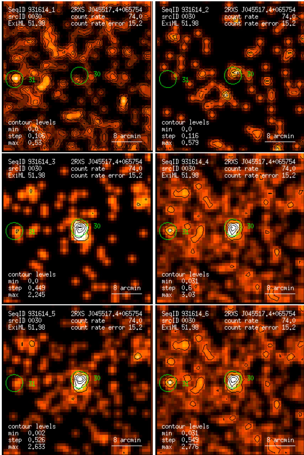
Figure 30: RASS 931614: detection 0030: band rate images, Gaussian filter: (1) PSPC channels 11 – 41, (2) 52 – 90, (3) 91 – 201, (4) 11 – 235, (5) 52 – 201, (6) 11 – 201. Broad band rates in counts/ks. Band rate contour levels in counts/ks/arcmin 2 .
