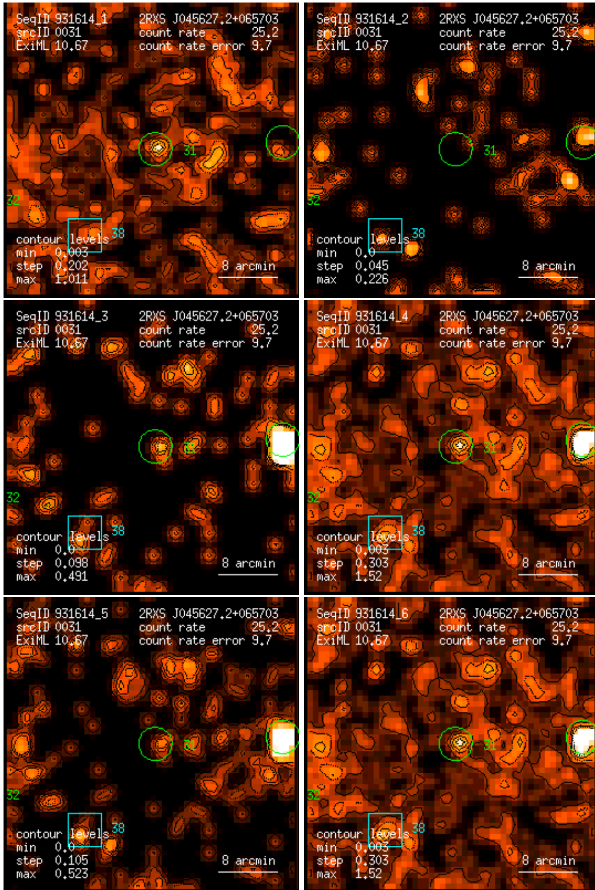
Figure 31: RASS 931614: detection 0031: band rate images, Gaussian filter: (1) PSPC channels 11 – 41, (2) 52 – 90, (3) 91 – 201, (4) 11 – 235, (5) 52 – 201, (6) 11 – 201. Broad band rates in counts/ks. Band rate contour levels in counts/ks/arcmin 2 .
