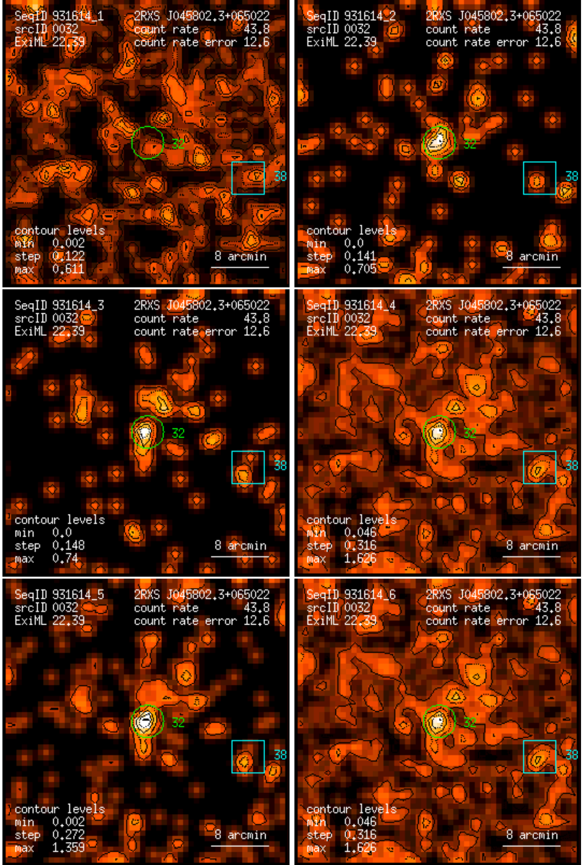
Figure 32: RASS 931614: detection 0032: band rate images, Gaussian filter: (1) PSPC channels 11 – 41, (2) 52 – 90, (3) 91 – 201, (4) 11 – 235, (5) 52 – 201, (6) 11 – 201. Broad band rates in counts/ks. Band rate contour levels in counts/ks/arcmin 2 .
