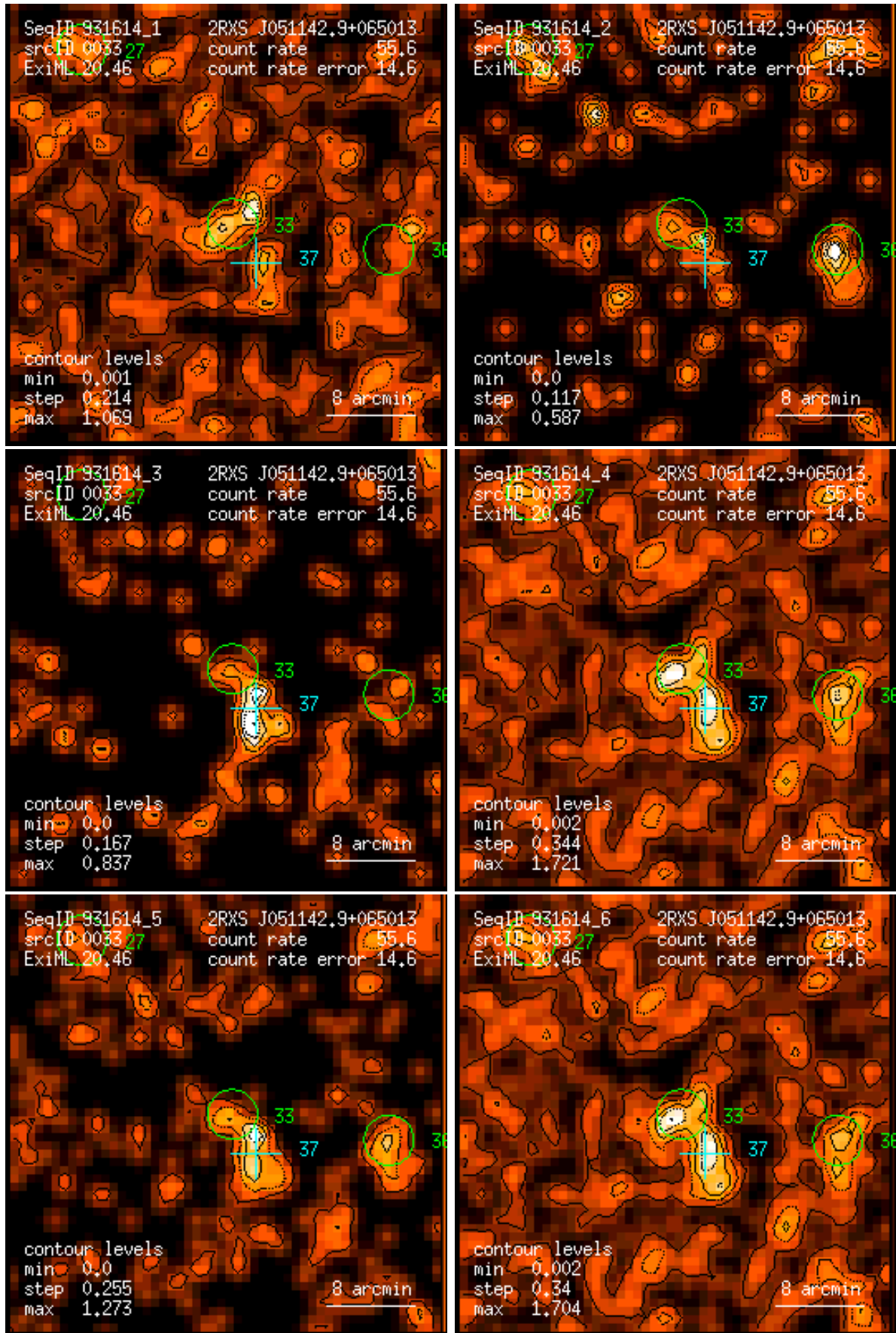
Figure 33: RASS 931614: detection 0033: band rate images, Gaussian filter: (1) PSPC channels 11 – 41, (2) 52 – 90, (3) 91 – 201, (4) 11 – 235, (5) 52 – 201, (6) 11 – 201. Broad band rates in counts/ks. Band rate contour levels in counts/ks/arcmin 2 .
