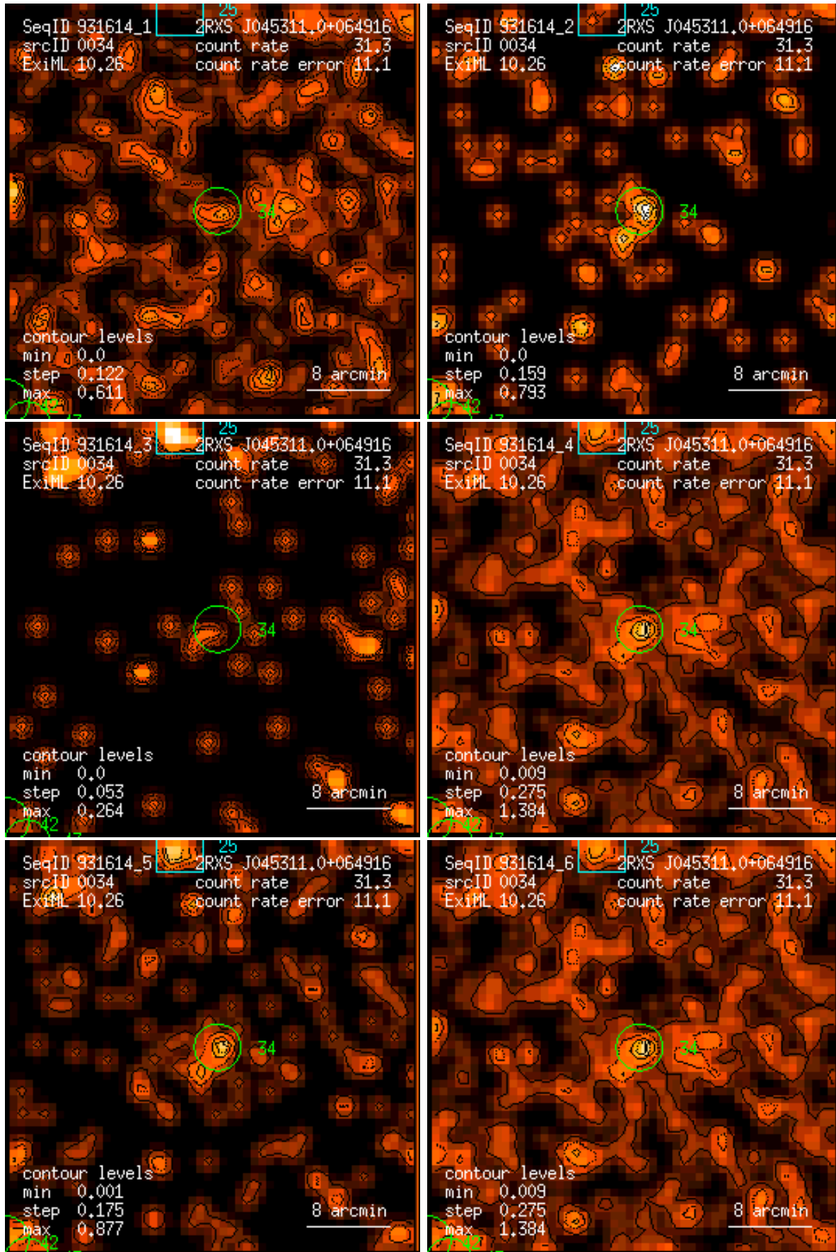
Figure 34: RASS 931614: detection 0034: band rate images, Gaussian filter: (1) PSPC channels 11 – 41, (2) 52 – 90, (3) 91 – 201, (4) 11 – 235, (5) 52 – 201, (6) 11 – 201. Broad band rates in counts/ks. Band rate contour levels in counts/ks/arcmin 2 .
