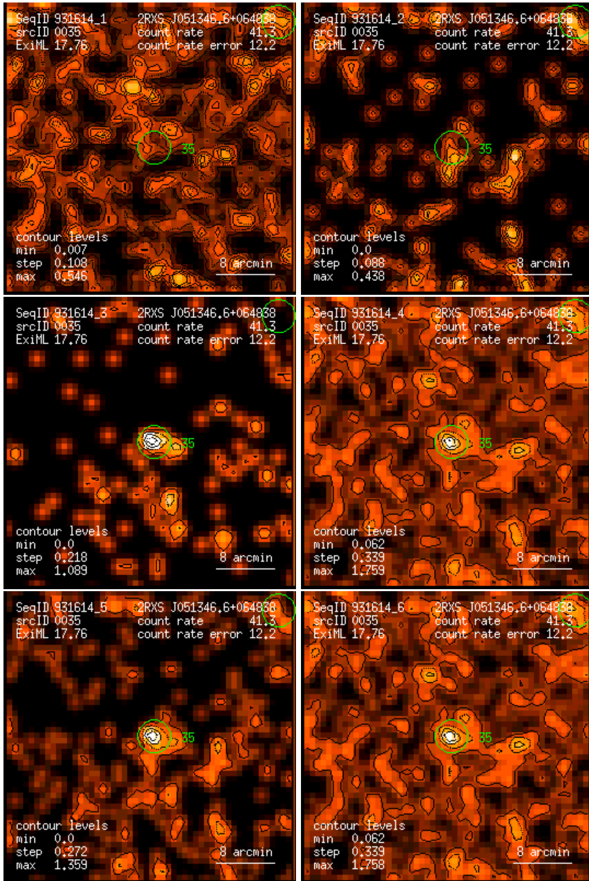
Figure 35: RASS 931614: detection 0035: band rate images, Gaussian filter: (1) PSPC channels 11 – 41, (2) 52 – 90, (3) 91 – 201, (4) 11 – 235, (5) 52 – 201, (6) 11 – 201. Broad band rates in counts/ks. Band rate contour levels in counts/ks/arcmin 2 .
