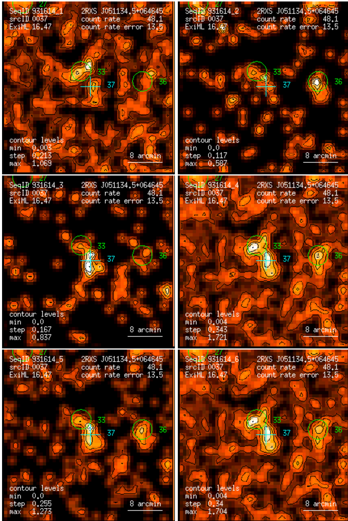
Figure 37: RASS 931614: detection 0037: band rate images, Gaussian filter: (1) PSPC channels 11 – 41, (2) 52 – 90, (3) 91 – 201, (4) 11 – 235, (5) 52 – 201, (6) 11 – 201. Broad band rates in counts/ks. Band rate contour levels in counts/ks/arcmin 2 .
