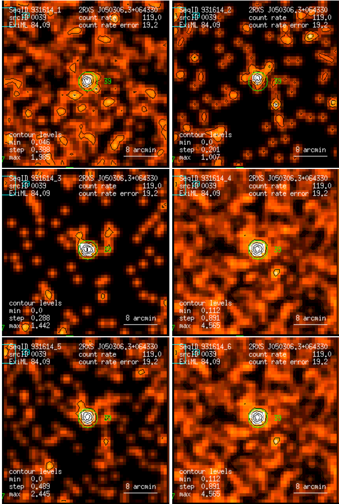
Figure 39: RASS 931614: detection 0039: band rate images, Gaussian filter: (1) PSPC channels 11 – 41, (2) 52 – 90, (3) 91 – 201, (4) 11 – 235, (5) 52 – 201, (6) 11 – 201. Broad band rates in counts/ks. Band rate contour levels in counts/ks/arcmin 2 .
