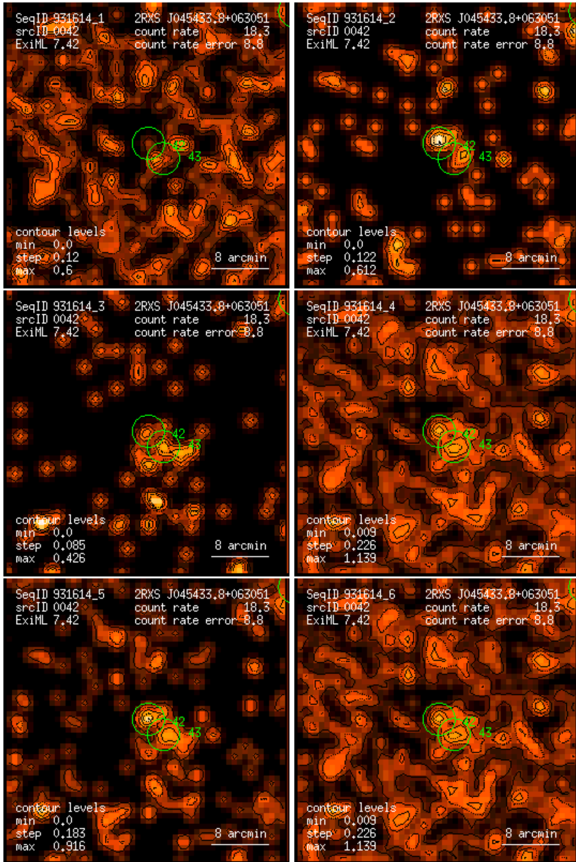
Figure 42: RASS 931614: detection 0042: band rate images, Gaussian filter: (1) PSPC channels 11 – 41, (2) 52 – 90, (3) 91 – 201, (4) 11 – 235, (5) 52 – 201, (6) 11 – 201. Broad band rates in counts/ks. Band rate contour levels in counts/ks/arcmin 2 .
