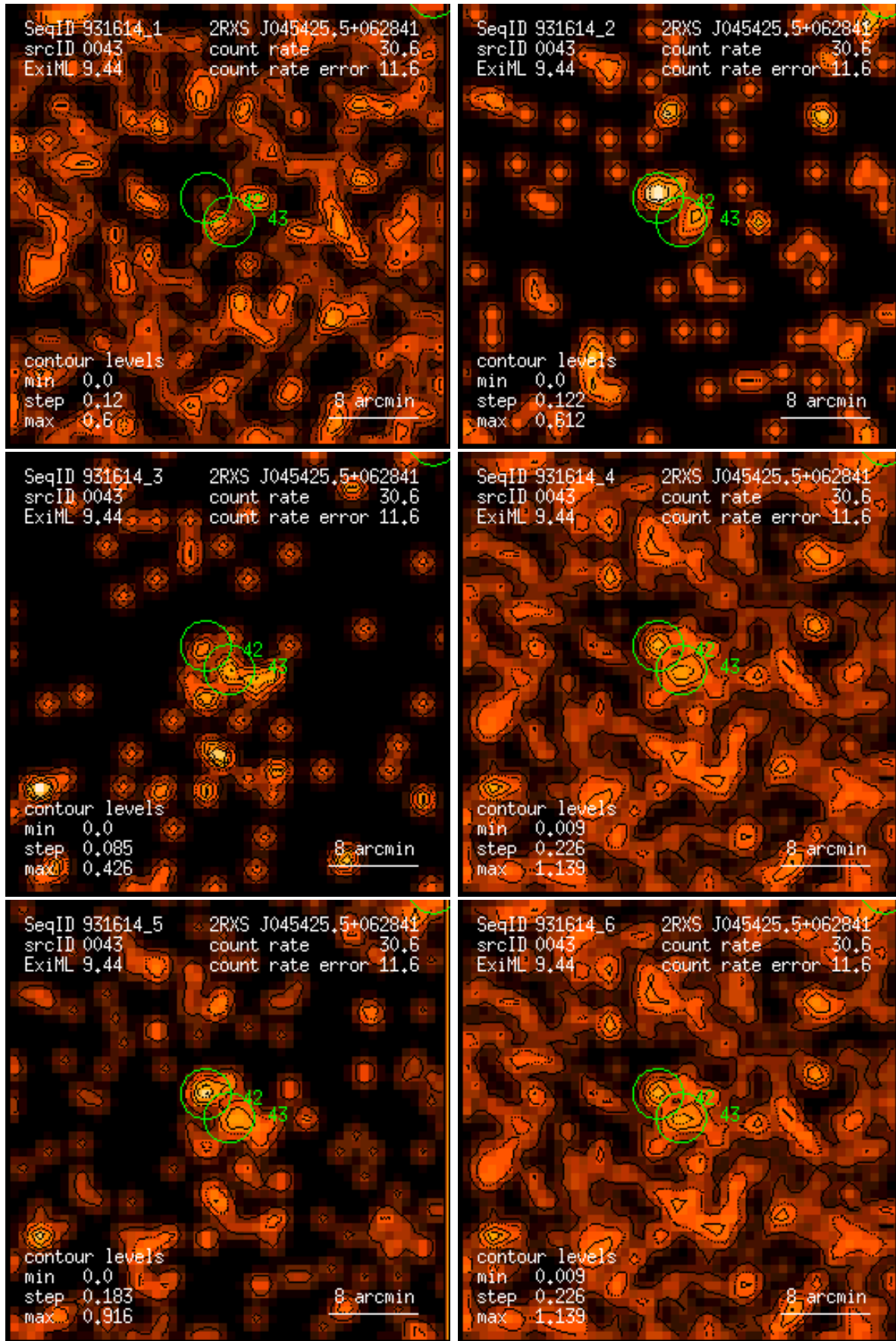
Figure 43: RASS 931614: detection 0043: band rate images, Gaussian filter: (1) PSPC channels 11 – 41, (2) 52 – 90, (3) 91 – 201, (4) 11 – 235, (5) 52 – 201, (6) 11 – 201. Broad band rates in counts/ks. Band rate contour levels in counts/ks/arcmin 2 .
