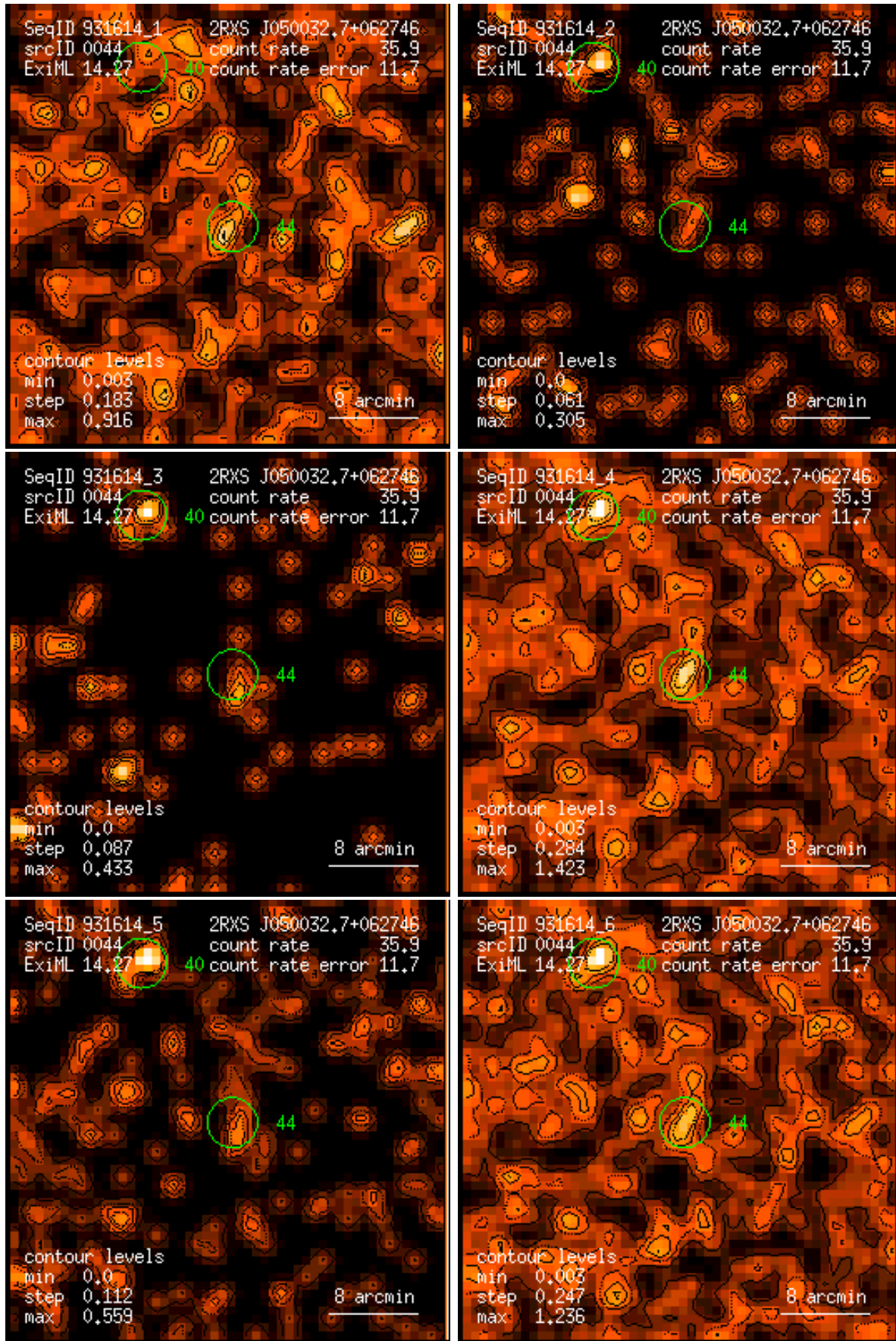
Figure 44: RASS 931614: detection 0044: band rate images, Gaussian filter: (1) PSPC channels 11 – 41, (2) 52 – 90, (3) 91 – 201, (4) 11 – 235, (5) 52 – 201, (6) 11 – 201. Broad band rates in counts/ks. Band rate contour levels in counts/ks/arcmin 2 .
