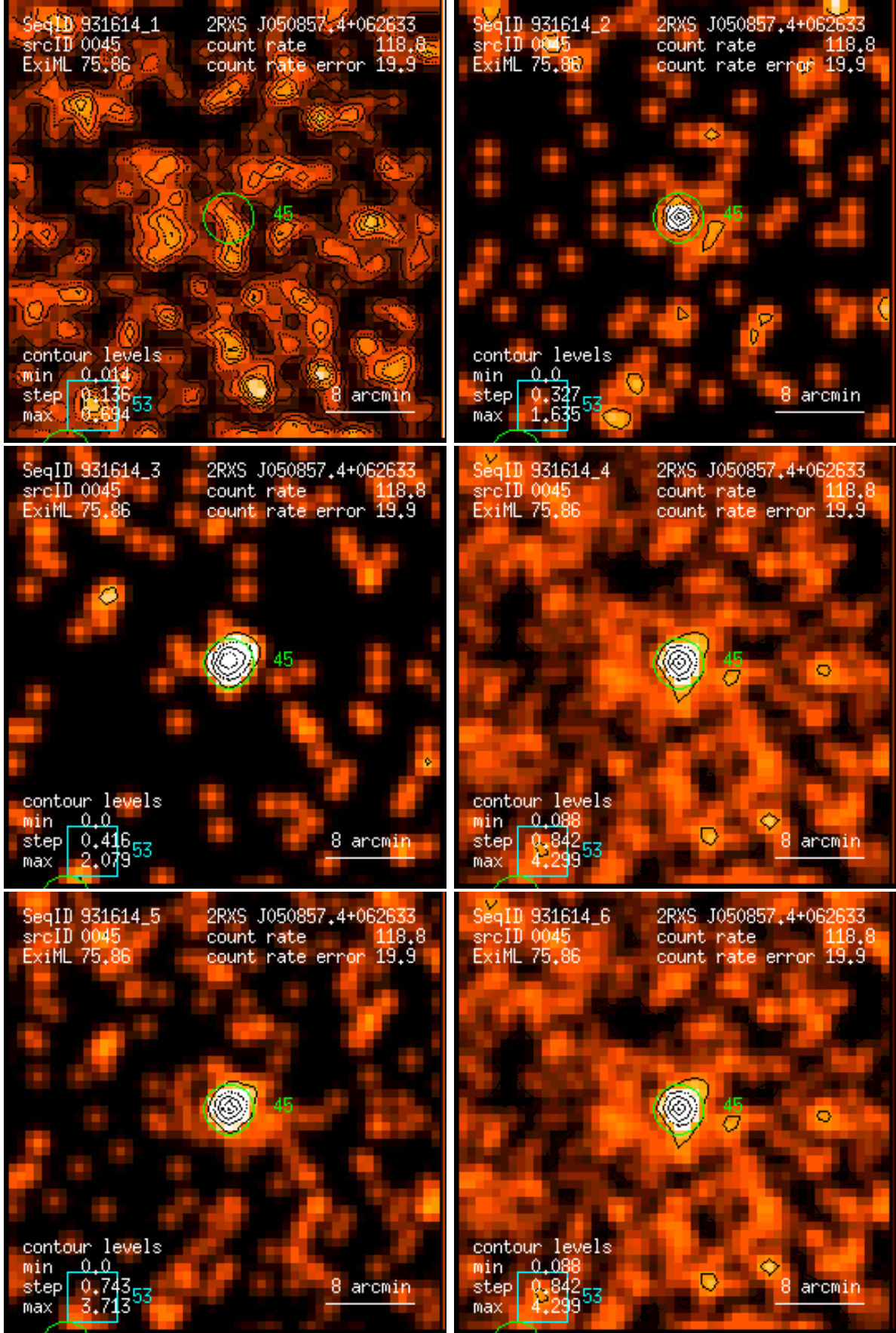
Figure 45: RASS 931614: detection 0045: band rate images, Gaussian filter: (1) PSPC channels 11 – 41, (2) 52 – 90, (3) 91 – 201, (4) 11 – 235, (5) 52 – 201, (6) 11 – 201. Broad band rates in counts/ks. Band rate contour levels in counts/ks/arcmin 2 .
