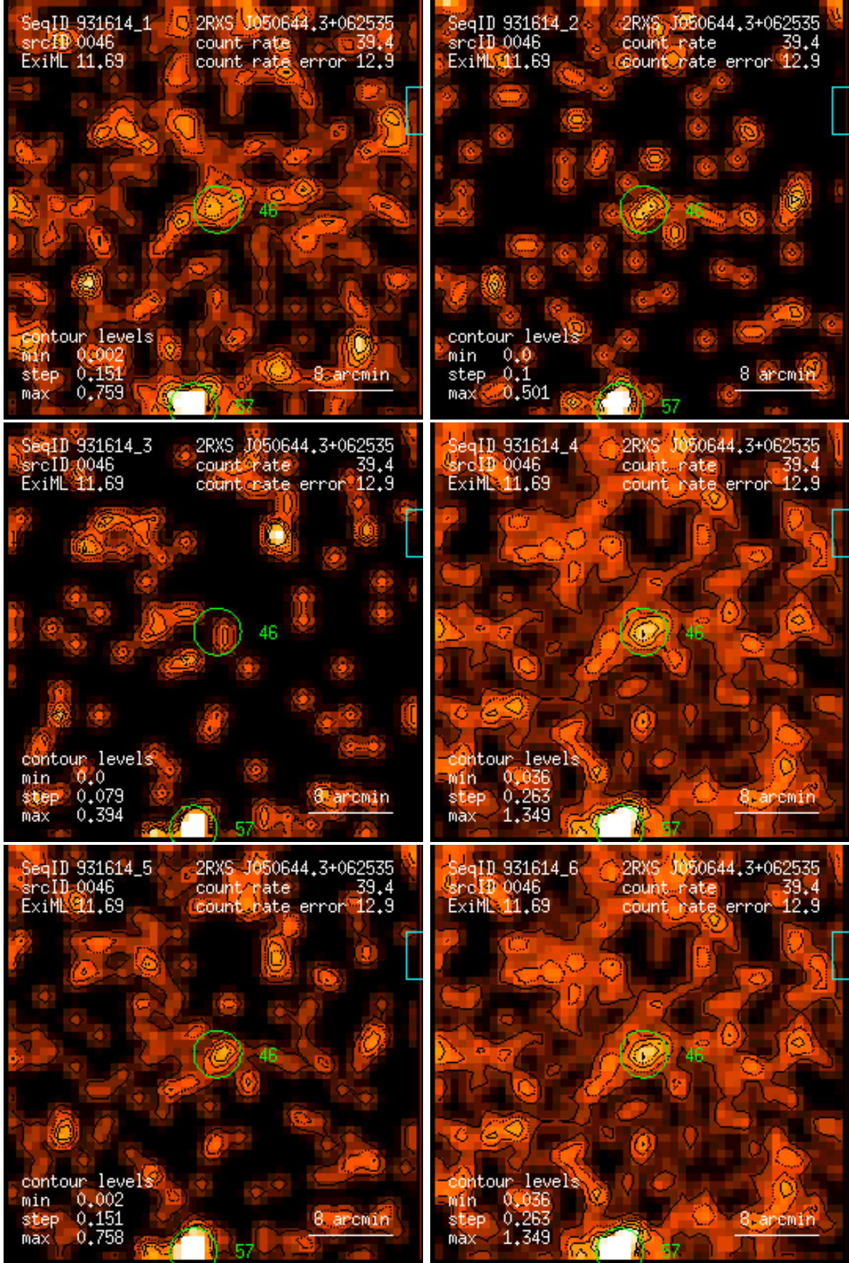
Figure 46: RASS 931614: detection 0046: band rate images, Gaussian filter: (1) PSPC channels 11 – 41, (2) 52 – 90, (3) 91 – 201, (4) 11 – 235, (5) 52 – 201, (6) 11 – 201. Broad band rates in counts/ks. Band rate contour levels in counts/ks/arcmin 2 .
