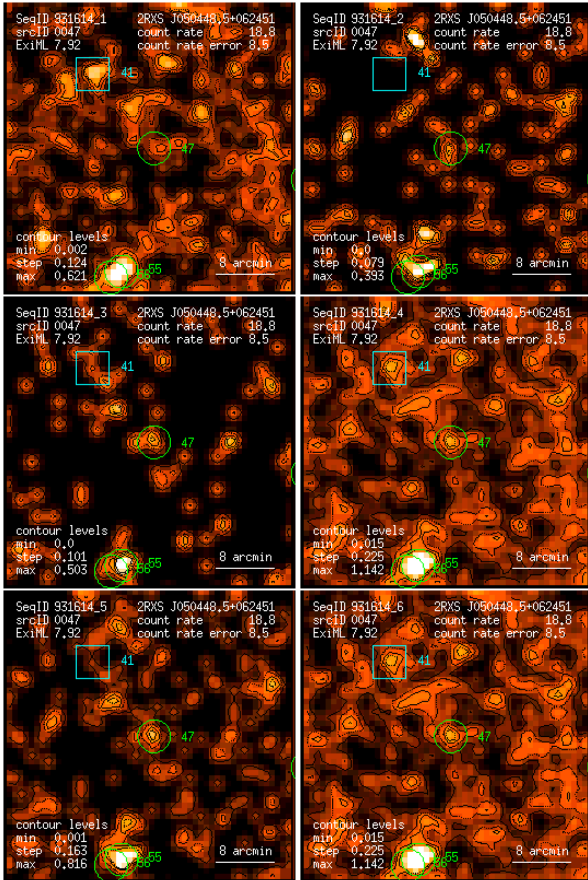
Figure 47: RASS 931614: detection 0047: band rate images, Gaussian filter: (1) PSPC channels 11 – 41, (2) 52 – 90, (3) 91 – 201, (4) 11 – 235, (5) 52 – 201, (6) 11 – 201. Broad band rates in counts/ks. Band rate contour levels in counts/ks/arcmin 2 .
