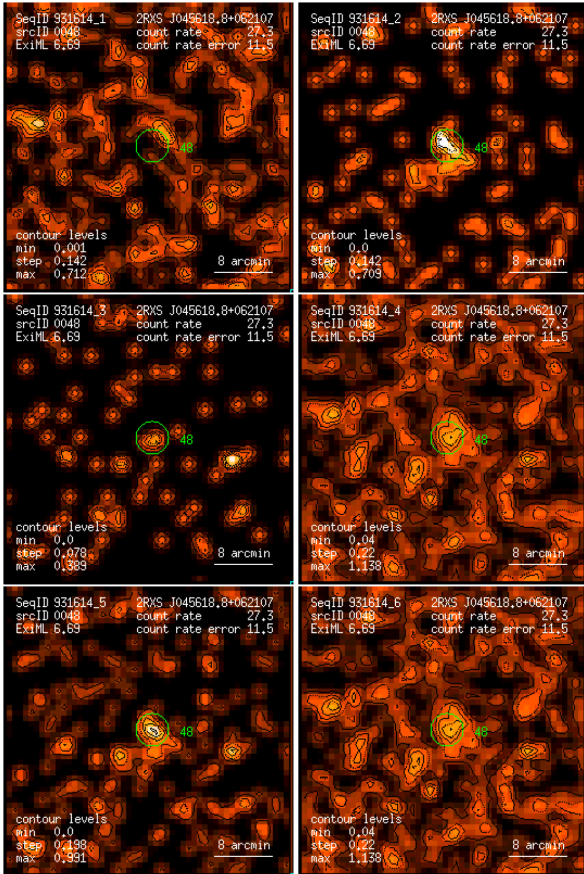
Figure 48: RASS 931614: detection 0048: band rate images, Gaussian filter: (1) PSPC channels 11 – 41, (2) 52 – 90, (3) 91 – 201, (4) 11 – 235, (5) 52 – 201, (6) 11 – 201. Broad band rates in counts/ks. Band rate contour levels in counts/ks/arcmin 2 .
