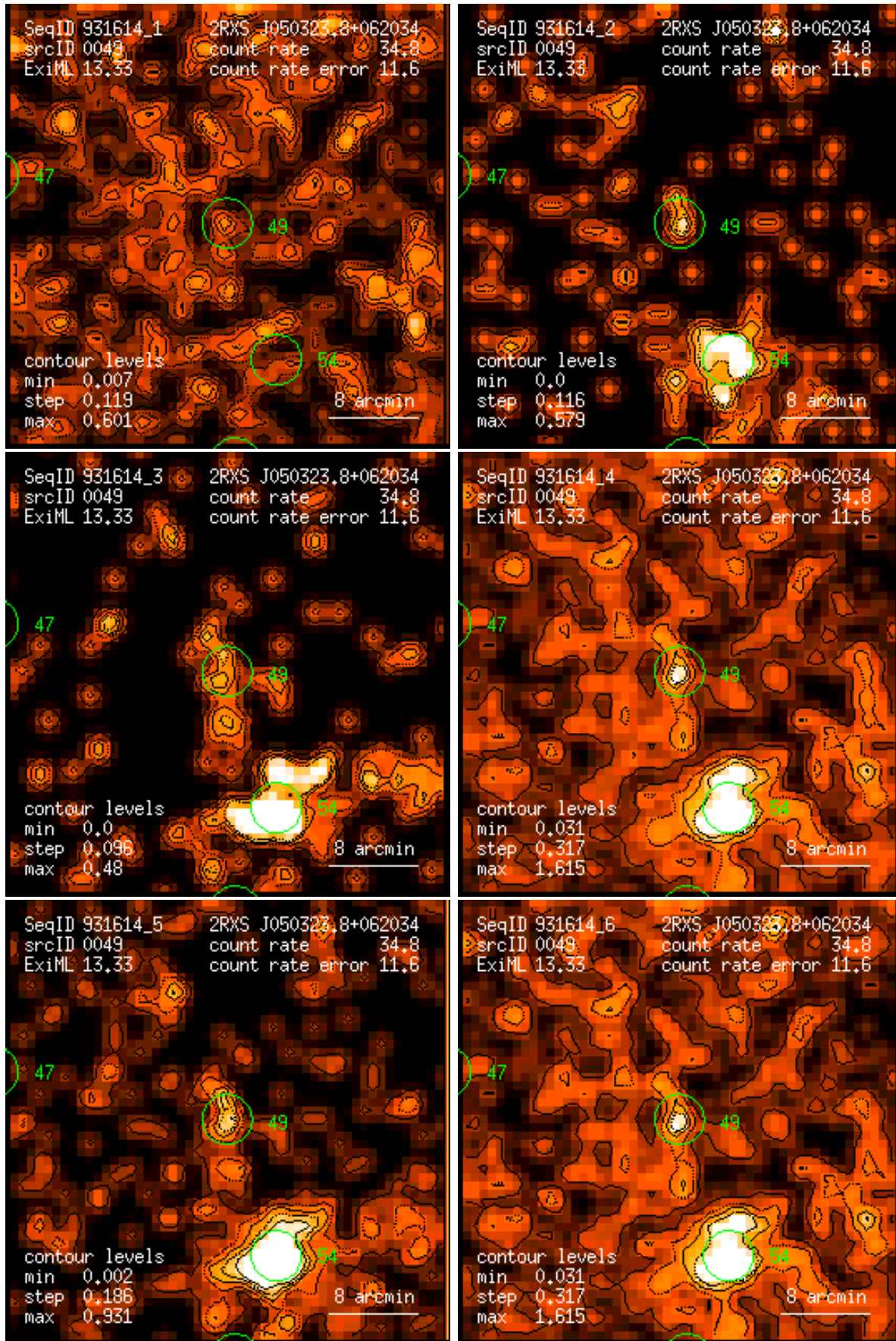
Figure 49: RASS 931614: detection 0049: band rate images, Gaussian filter: (1) PSPC channels 11 – 41, (2) 52 – 90, (3) 91 – 201, (4) 11 – 235, (5) 52 – 201, (6) 11 – 201. Broad band rates in counts/ks. Band rate contour levels in counts/ks/arcmin 2 .
