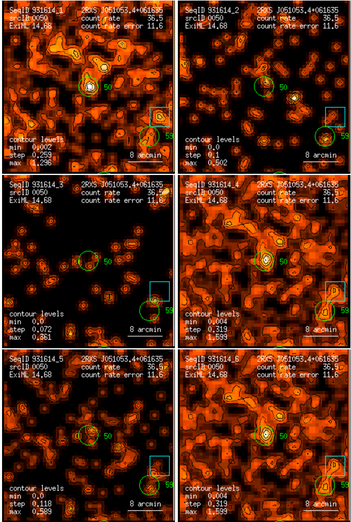
Figure 50: RASS 931614: detection 0050: band rate images, Gaussian filter: (1) PSPC channels 11 – 41, (2) 52 – 90, (3) 91 – 201, (4) 11 – 235, (5) 52 – 201, (6) 11 – 201. Broad band rates in counts/ks. Band rate contour levels in counts/ks/arcmin 2 .
